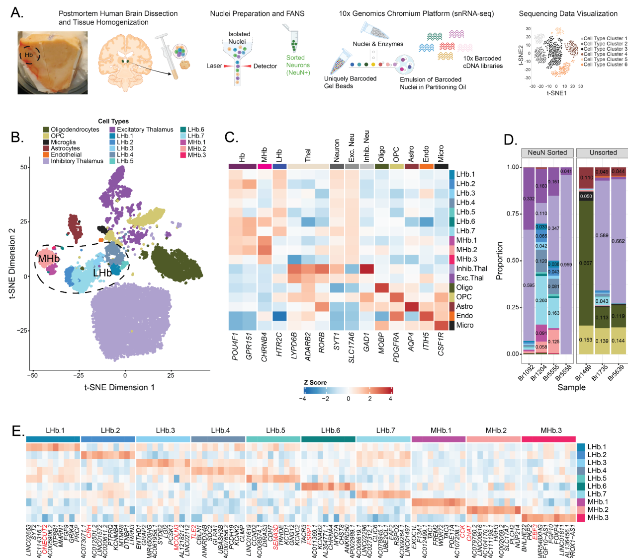
Fig. 1. Single cell transcriptomic atlas of the human habenula (Hb). A ) Overview of nuclei preparation and single nucleus RNA-sequencing (snRNA-seq) data generation using the 10x Genomics Chromium Single Cell Gene Expression platform B ) t-SNE plot of 16,437 quality-controlled single nucleus transcriptomes (colored by cell type) from the epithalamus of 7 neurotypical control donors. Dashed circle highlights lateral (L) and medial (M) Hb cell type clusters (n=2,214 LHb and n=710 MHb nuclei). C ) Heatmap depicting expression of known marker genes (x-axis) that were used to annotate broad cell types as well as habenula vs. thalamic neurons. The color of each square (blue to red) indicates z-scored relative expression of the corresponding marker gene. D ) Proportion plot displaying cell type composition of each sample. NeuN+ sorted samples were enriched for neurons and therefore contain more neuronal cell types. E ) Heatmap highlighting the top 10 mean ratio marker genes (x-axis) for each identified LHb and MHb neuronal subpopulation. The color of each square (blue to red)
