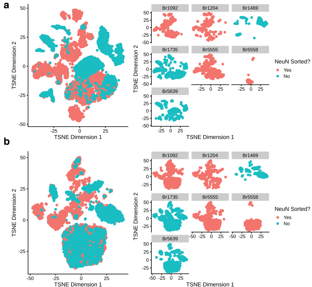
Fig. S5. Pre and post harmony by NeuN sorting. Batch correction of snRNA-seq data visualized by t-SNE plots. A) t-SNE of principal components (PCs) pre-batch correction, colored by neuronal enrichment performed with NeuN antibody labeling and FANS. B) t-SNE of PCs post-batch correction with Harmony , colored by neuronal enrichment performed with NeuN antibody labeling and FANS. While batch correction with Harmony reduced NeuN sorting differences, some differences remain. This is expected given that the NeuN sorted samples are enriched for neuronal cell types compared to samples without NeuN sorting.
