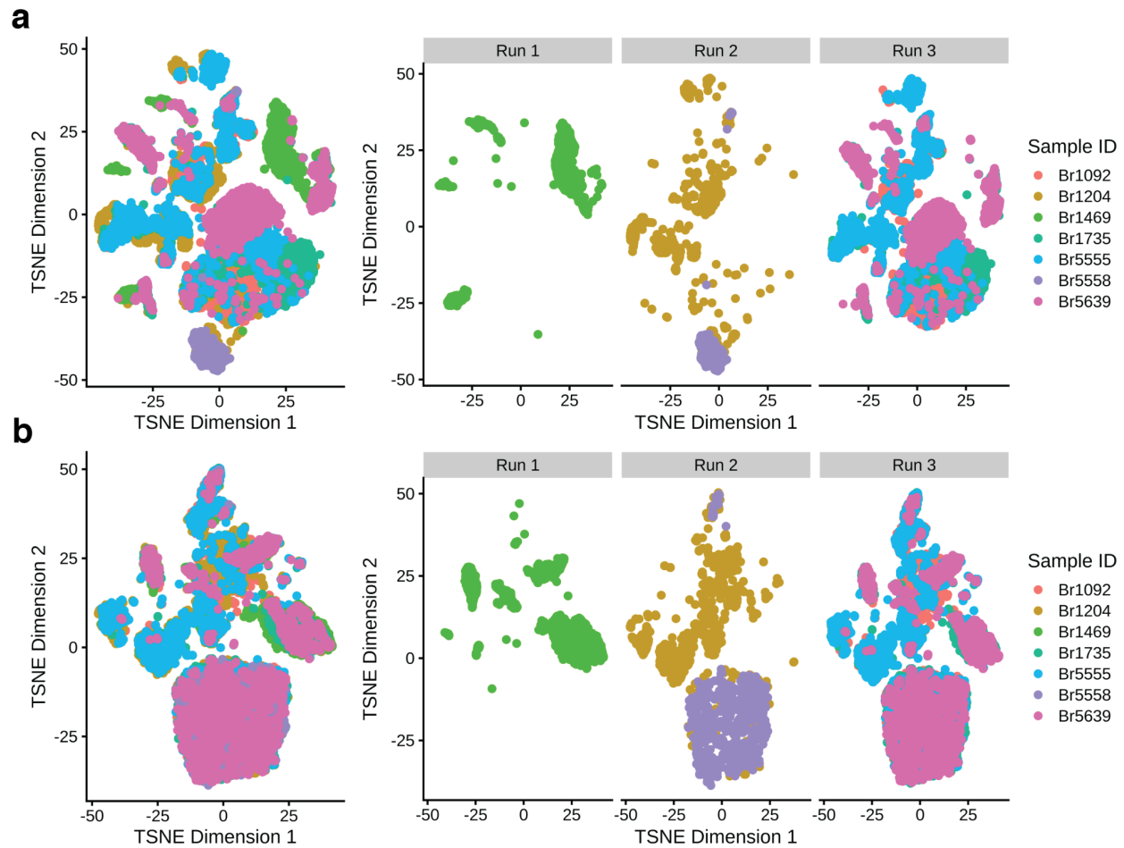
Fig. S4. Pre and post harmony by sequencing run. Batch correction of snRNA-seq data visualized by t-SNE plots. A) t-SNE of principal components (PCs) pre-batch correction, colored by sample and faceted by sequencing run. B) t-SNE of PCs post-batch correction with Harmony , colored by sample and faceted by sequencing run. Batch correction with Harmony reduced sample and sequencing run batch effects.
