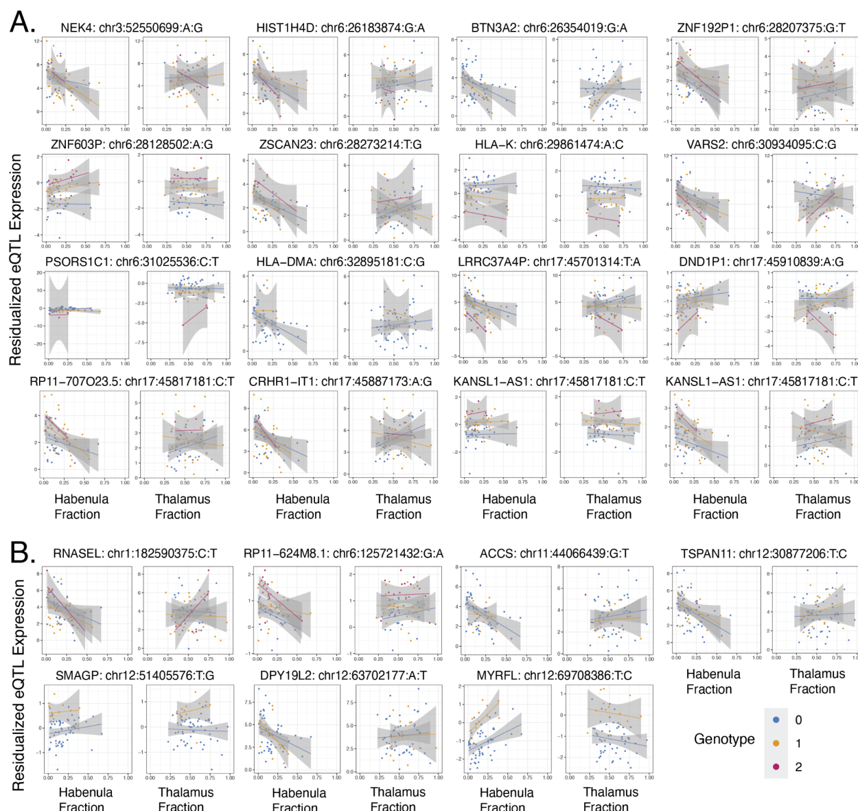
Fig. S20. Habenula and thalamus neuronal cell fraction interaction with SNP alleles for independent eQTLs whose SNPs are SCZD risk SNPs or genes are DEGs. Scatterplots of residualized normalized expression compared against either the estimated habenula or the thalamus neuronal fractions ( T_{\text{ot.Hb}} and T_{\text{ot.Thal}} ) with SNP allele regression lines colored by allele (homozygous major allele in blue, heterozygous in orange, homozygous minor allele in red). In all SNP-gene pairs, the major allele matched the reference allele. A) Cell fraction interaction eQTLs could be computed for 14 of the 16 SNP-gene pairs from Hb-enriched thalamus independent eQTLs whose SNPs are PGC3 SCZD GWAS risk SNPs ( p < 5 \times 10^{-8} ). B) SNP-gene pairs from Hb-enriched thalamus independent eQTLs whose genes were SCZD DEGs (FDR < 0.1). Related to Fig. 5C .
