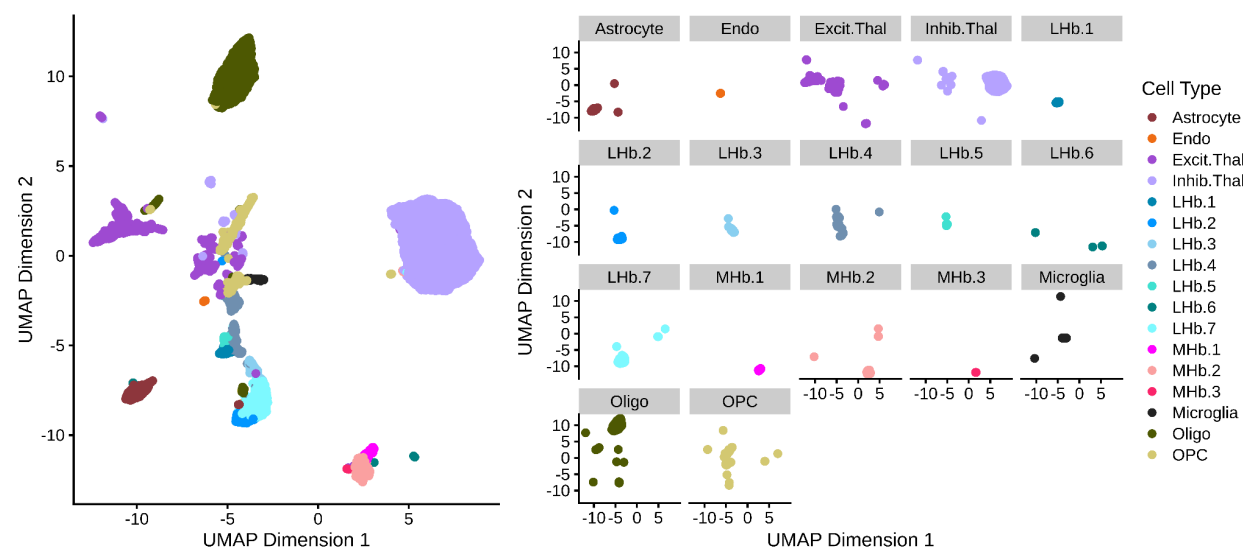
Fig. S14. UMAP representation of the snRNA-seq data. Post-QC snRNA-seq data visualized using UMAP (similar to Fig. 1), colored by cell type. The right side shows the UMAP faceted by cell type.
