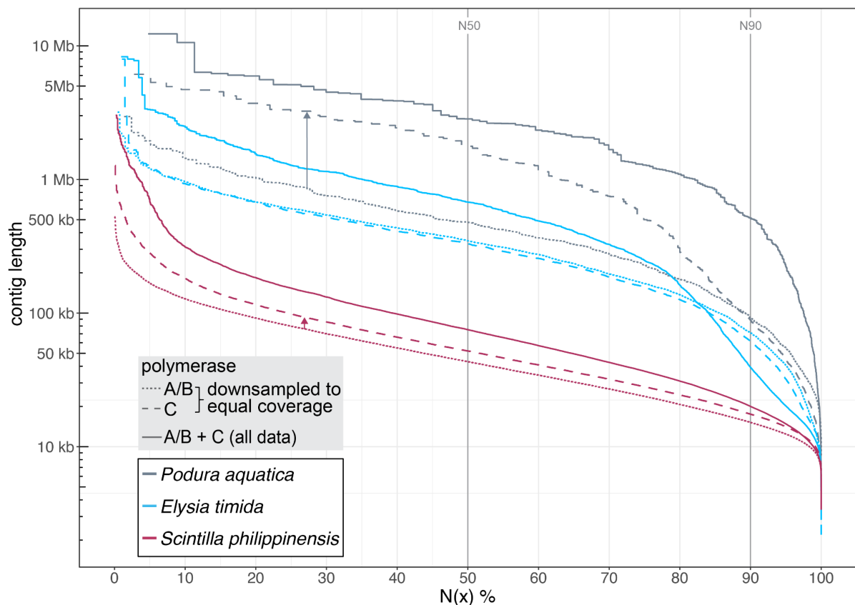
Figure 5: Impact of polymerase C on assemblies of mollusc and collembola species. Assembly contiguity visualized as N(x) graphs that show contig sizes on the Y-axis, for which x percent of the assembly consists of contigs of at least that size (N50 and N90 values are indicated). Assemblies are generated with an equal (downsampled) coverage of reads from polymerase A/B (dotted lines) and C (dashed lines). Assemblies generated with all data are shown as solid lines. Colors refer to different species.
