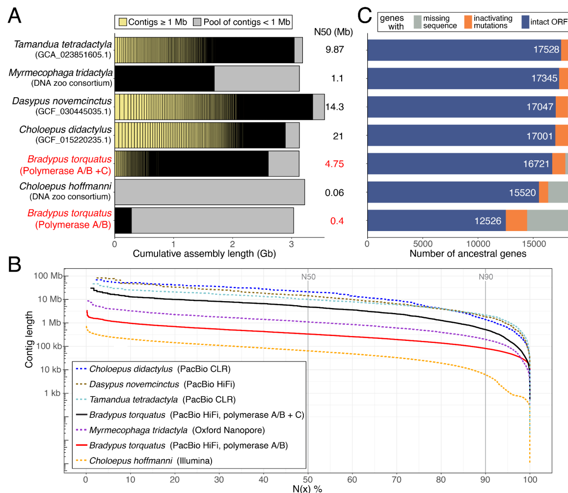
Figure 4: Comparison of xenarthran genome assemblies.
