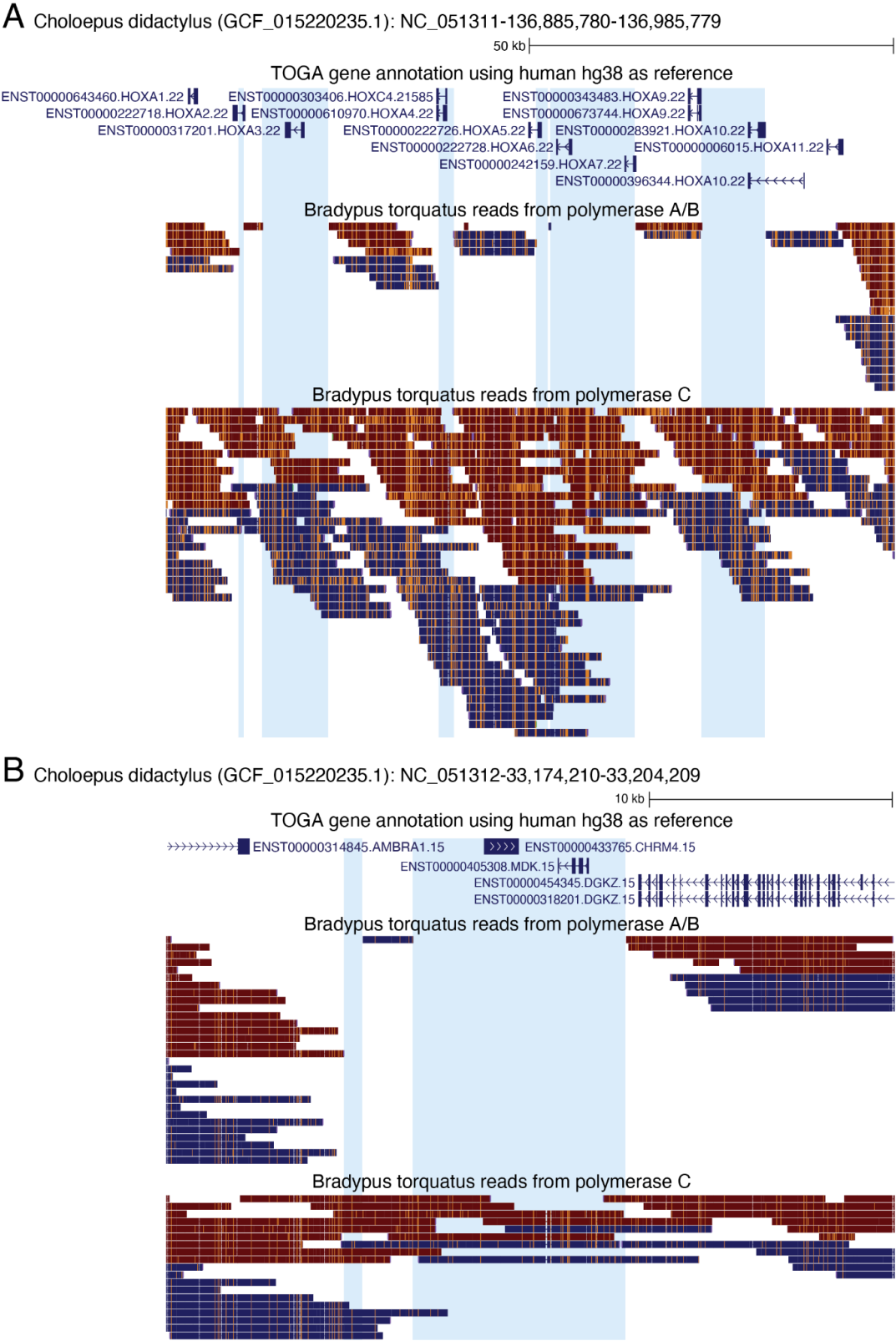
Figure 2: PCR bias in reads produced with polymerase A/B.
