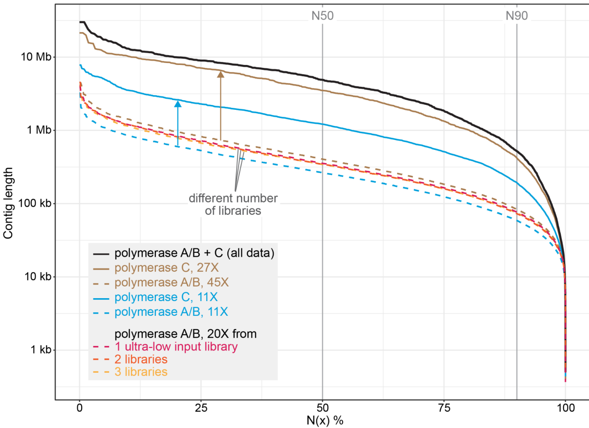
Figure 1: Contiguity of B. torquatus assemblies generated with data from ultra-low input libraries prepared with polymerases A/B and/or C at different coverages.
