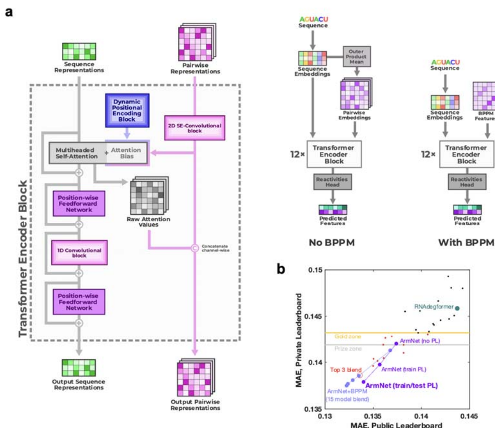
Extended Data Figure 8. ArmNet (Artificial Reactivity Mapping using neural Networks) post-competition model from the vigg team. (a) Two modifications to the Kaggle 1st place model improved performance: (1) adding the 1D convolutional module after each attention block, as was done in the Kaggle 2nd place solution, and (2) concatenating the attention scores and BPP features and combining them using the 2D convolutional layer of the next block. The second modification supports the idea from RibonanzaNet and the 3rd place solution – to provide two-way communication between the sequence and 2D features – is important for model performance. Triangular operations tested in RibonanzaNet were not included in ArmNet. (b) With input of BPP matrices from EternaFold and blending an increasing number of models (1, 3, 5, 7, 15), ArmNet outperforms all previous models in both private and public leaderboard MAE (light blue symbols). Without BPP and as a single model, ArmNet achieves excellent private leaderboard MAE when trained on pseudo labels from the 15-model ArmNet-BPPM ensemble ('PL'; purple). When the single no-BPP ArmNet model is instead trained on pseudolabels derived from the top 3 Kaggle submissions (as in RibonanzaNet; Extended Data Figure 7 ), MAE scores are slightly worse than other ArmNet models and RibonanzaNet (not shown; see Supplemental Table S5 ). MAE is mean absolute error to test data after clipping values between 0 and 1. 'Gold zone' and 'prize zone' mark 11th place and 6th place Kaggle scores which were cutoffs for Kaggle gold medals and prizes, respectively.
