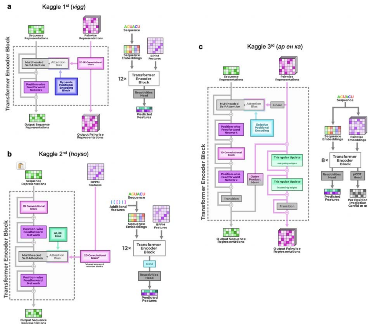
Extended Data Figure 6. Full architecture diagrams of top 3 Ribonanza Kaggle models. (a) 1st place model (team vigg ), (b) 2nd place model (team hoysa ), and (c) one of two models used for 3rd place submission (Twin Tower model from team ap eh ka ).
