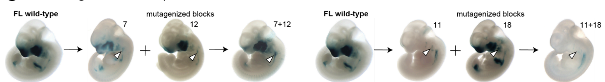
Supplementary Figure 8. Additional results of paired block mutagenesis. (A) Illustration of paired block mutagenesis outcomes for all possible combinations of loss and gain mutations. Bars represent ranges of possible outcomes that would be classified as additive or non-additive. (B) Additional additive pair examples. (C) Remaining non-additive pairs. Combined mutagenesis of enhancer FL blocks 7 and 12 resulted in higher branchial arch 3 activity, while no change in activity in these structures was observed in constructs with single block mutations (see also hindbrain activity). Combined mutagenesis of enhancer FL blocks 12 and 18 resulted in lower activity in branchial arch 2 compared to constructs mutated in block 12 only, while mutation of block 18 in isolation did not appreciably change the activity of this structure (compare also hindbrain activity). White arrowheads highlight structures of interest. Related to Figure 5.
