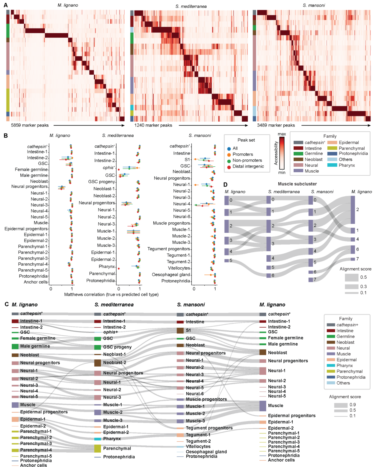
Figure S2. Loss of cell type specificity in conserved accessibility patterns, related to Figure
