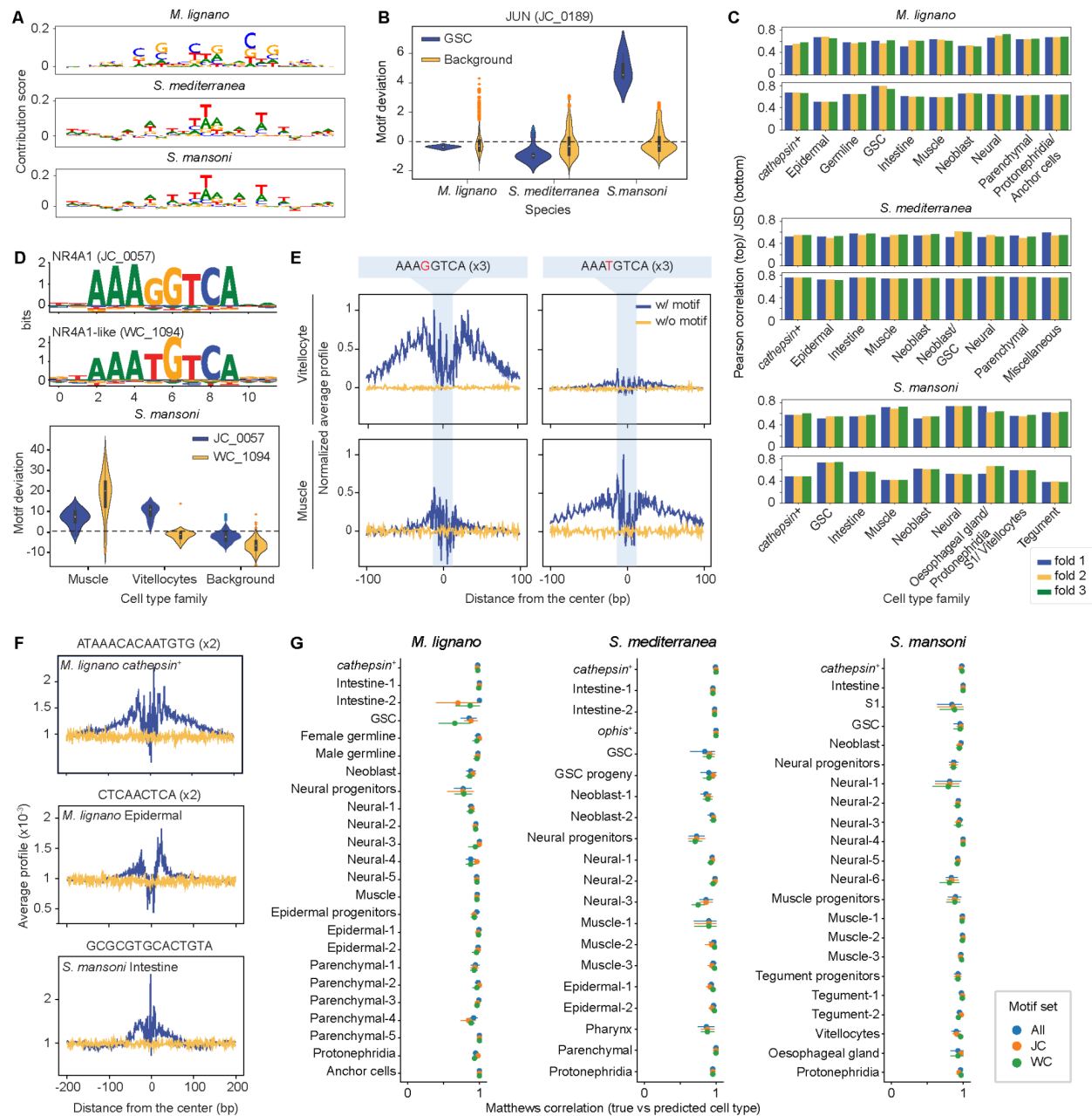
Figure S3. ChromBPNet models learn the sequence features dictating ATACseq signal, related to Figure 2
