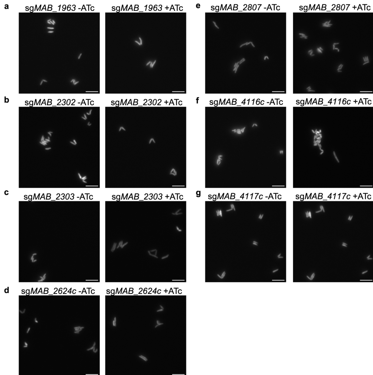
Extended Data Fig. 4: Membrane transporter mutants do not display gross morphological changes.
