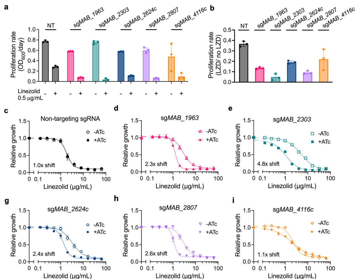
Figure 2: Knockdown of membrane transporters increases sensitivity to linezolid.
