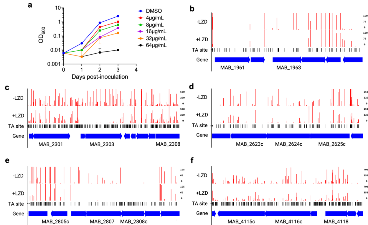
Extended Data Fig. 2: TnSeq screening in clinical isolate BWH-F reveals determinants of linezolid resistance.
