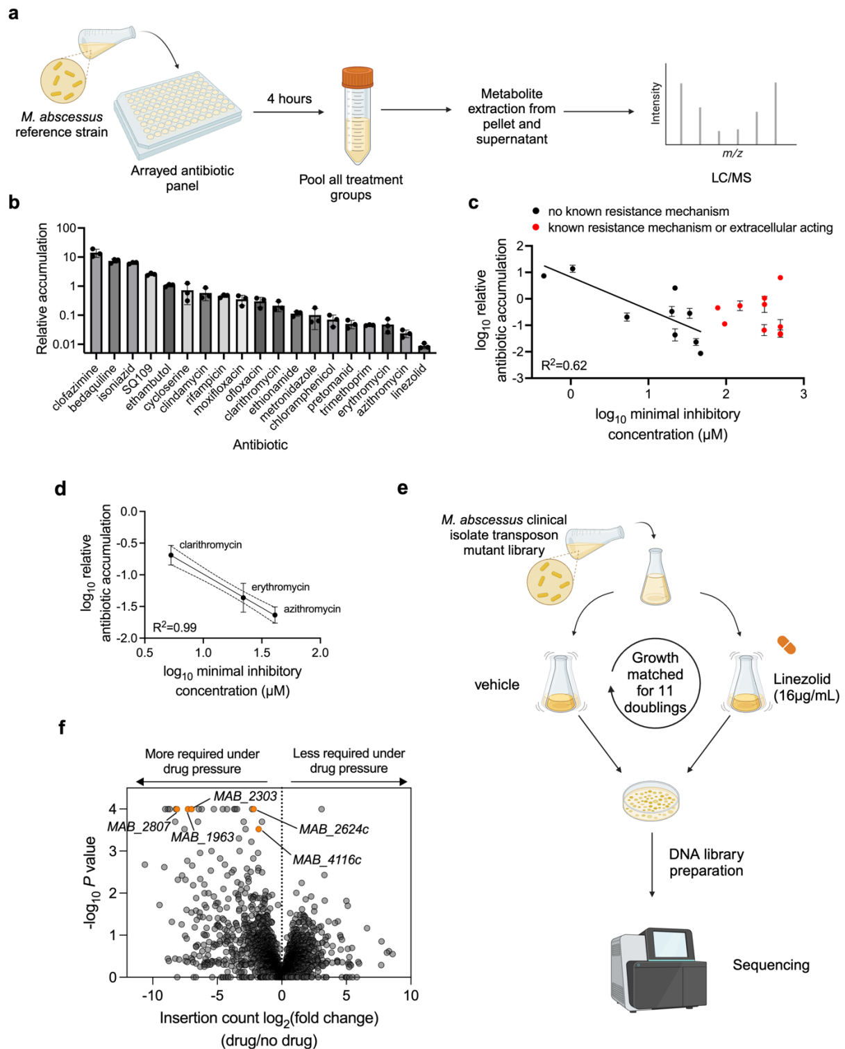
Figure 1: TnSeq reveals differential requirement of numerous membrane transporters with linezolid exposure.
