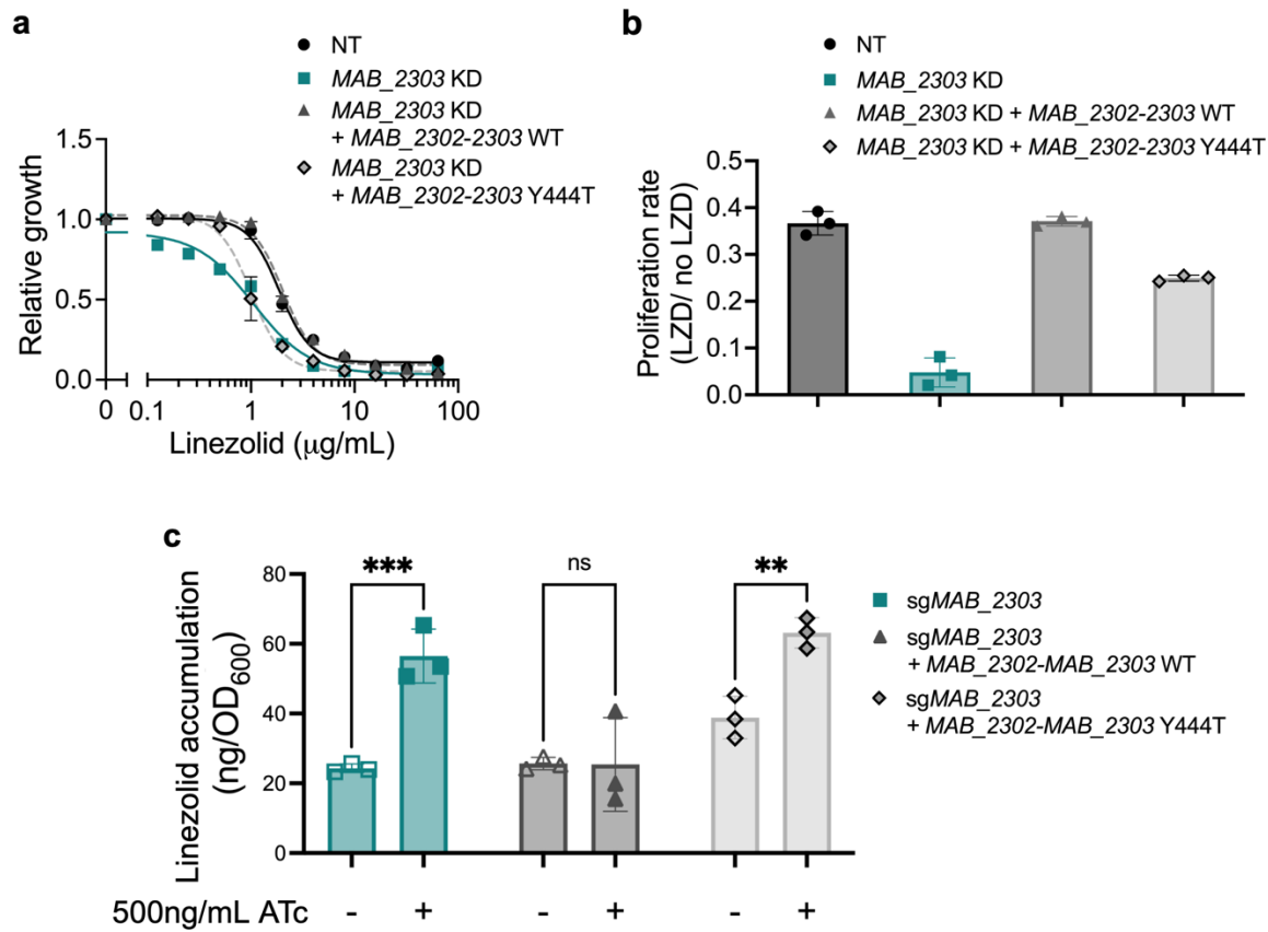
Figure 4. MAB_2303 effluxes linezolid.
