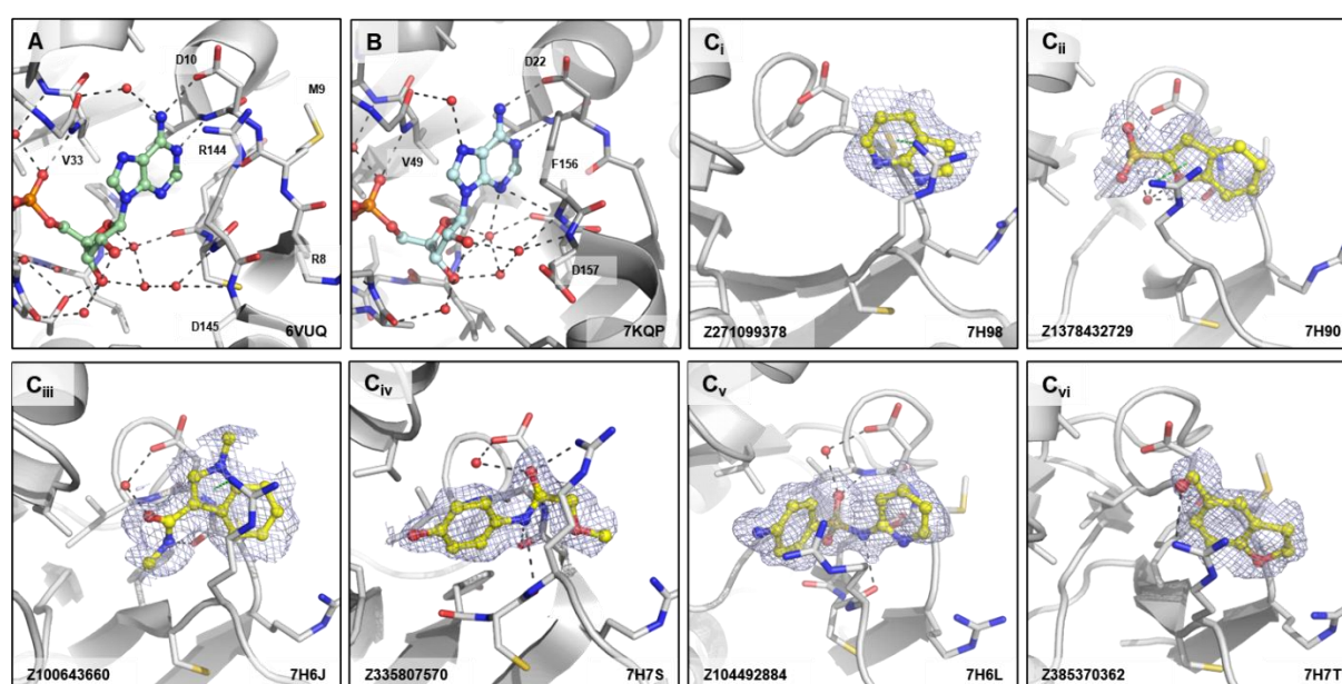
Figure 8. Fragments binding to the Arg144 pocket of CHIKV nsP3 macrodomain.
