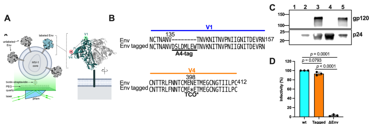
Fig 2. Engineering HIV-1 CRF01_AE Env for site-specific fluorescent labeling. (A) Schematic of the smFRET imaging assay. Pseudovirions with HIV-1 CRF01_AE Env (strain 92TH023) containing a single labeled gp120 domain were immobilized on quartz slides and imaged using TIRF microscopy. (B) Sequence alignments indicating sites of A4 peptide insertion into the V1 loop and TCO* substitution in the V4 loop for fluorophore attachment. (C) Qualitative detection of the indicated proteins from purified pseudovirions with HIV-1 CRF01_AE Env through immunoblots. Lane 1, mock-produced virus; lane 2, ΔEnv virions; lane 3, wild-type Env pseudotyped virions; lane 4, Env V1-A4/V4-TAG (tagged) pseudotyped virions produced in the absence of the TCO* amino acid; lane 5, tagged Env pseudovirions produced in the presence of the TCO* amino acid. (D) Infectivity of lentiviruses with either wild-type HIV-1 CRF01_AE Env (wt), V1-A4/V4-TAG Env (tagged), or bald particles was evaluated in TZM-bl cells. Infectivity values are expressed as the percentage of wild-type Env and normalized to the expression level of gp120 and p24. Each point indicates the arithmetic mean of three technical replicates. Bars represent the average of three independent experiments per condition. Error bars reflect the standard error. The statistical significance was evaluated through parametric t -tests. p -values are indicated and those <0.05 were considered statistically significant.
