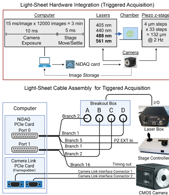
Suppl. Fig. 1. Hardware wiring diagram of the light-sheet microscope. Hardware integration (top panel) for camera-triggered activation of the excitation lasers and piezo z-stage that limits communication to a single instruction from the computer every 3 minutes. Wiring diagram (bottom panel): two Nikon ‘standard cables’ connect to the NiDAQ card installed in the computer. These two cables link to the laser control box, stage controller and camera. The images captured are received by the computer through a camera link PCIe card. and
