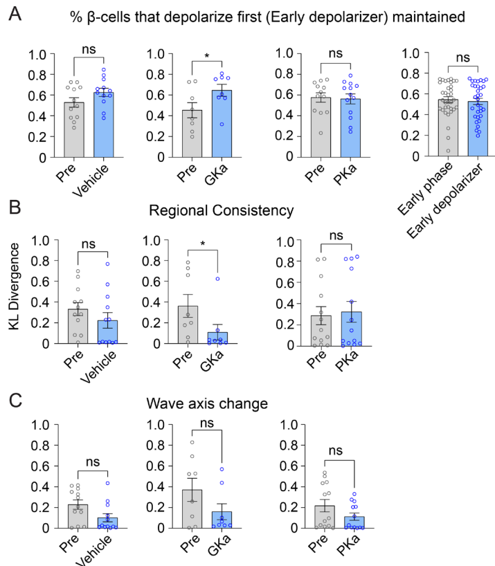
Suppl. Fig. 5. Effect of glycolytic activators on the \beta -cells that depolarize first. (A-C) Effect of vehicle, glucokinase activator (GKa), and pyruvate kinase activator (PKa) on the retention (A), regional consistency (B), and wave axis change (C) of the \beta -cells that depolarize first (Early depolarizer). The retention of \beta -cells that depolarize first (Early depolarizer) is similar to cells that depolarize and repolarize first (Early phase). Data are displayed as mean \pm SEM.
