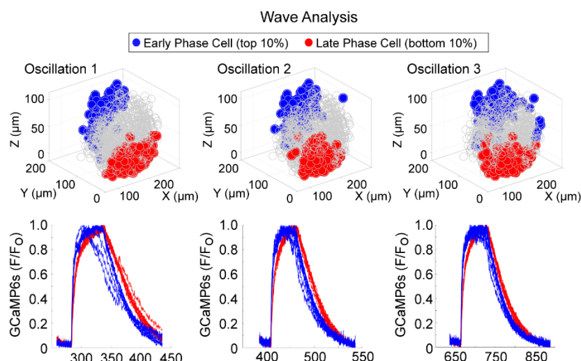
Suppl. Fig. 3. Location of early and late phase cells in an islet with stable wave axis. 3D representation of the islet showing the location of early phase cells (blue) and late phase cells (red) over three consecutive oscillations (top panel) and their corresponding \text{Ca}^{2+} traces (bottom panel).
