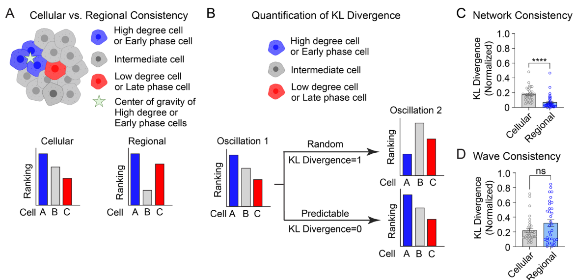
Fig. 4. Cellular and regional consistency of the \beta -cell network and \text{Ca}^{2+} wave quantified by KL divergence. (A) Schematic showing cellular consistency analysis and regional consistency analysis. (B) Schematic depicting the use of KL divergence to determine consistency between consecutive oscillations. Every \beta -cell in the islet is ranked, with near-zero KL divergence values indicating high consistency between oscillations and near-unity KL divergence indicating randomness. (C-D) Comparison of cellular vs. regional consistency of the network (C) and wave (D) by KL divergence. Data are displayed as mean \pm SEM. **** P < 0.0001 by normality test followed by Paired Student's t-test or Wilcoxon Signed-Rank Test.
