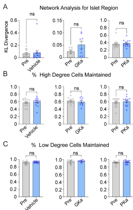
Suppl. Fig. 4. Effect of glycolytic activators on the \beta -cell network. (A-C) Effect of vehicle, glucokinase activator (GK \alpha ), and pyruvate kinase activator (PK \alpha ) on regional consistency of the \beta -cell network (A), high degree cell retention (B), and low degree cells retention (C). Data are displayed as mean \pm SEM.
