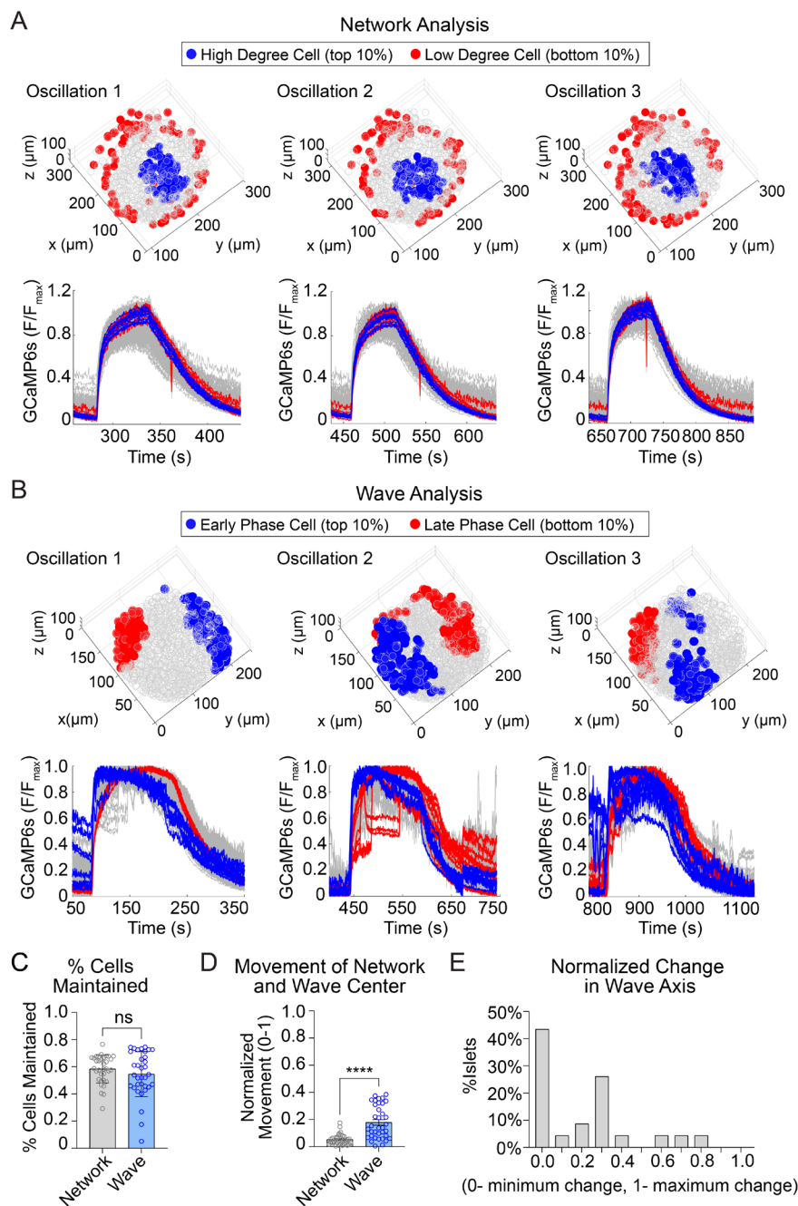
Fig. 3. The network of highly synchronized \beta -cells is consistent between oscillations, while the \text{Ca}^{2+} wave axis rotates. (A) 3D representation of the islet showing the location of high degree cells (blue) and low degree cells (red) over three consecutive oscillations (top panel) and their corresponding \text{Ca}^{2+} traces (bottom panel). (B) 3D representation of the islet showing the location of early phase cells (blue) and late phase cells (red) over three consecutive oscillations (top panel) and their corresponding \text{Ca}^{2+} traces (bottom panel). (C) Quantification of the retention rate of high degree and early phase cells. (D) Relative spatial change in the center of gravity of \beta -cell network vs. the \beta -cell \text{Ca}^{2+} wave. (E) Frequency distribution showing the normalized change in \text{Ca}^{2+} wave axis for all islets. Data are displayed as mean \pm SEM. **** P < 0.0001 by normality test followed by Paired Student's t-test or Wilcoxon Signed-Rank Test.
