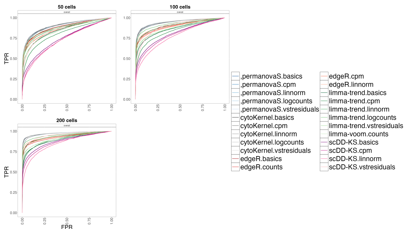
Figure 2: Receiver operating characteristic (ROC) curves generated using the distinct sensitivity (varying the number of cells) simulation design (Crowell et al., 2020; Tiberi et al., 2022). cytoKernel demonstrates better performance when varying the number of available cells. TPR versus FPR in muscat simulated data; with 50, 100 and 200 cells per cluster-sample combination, corresponding to a total of 900, 1800 and 3600 cells, respectively. Results are aggregated over the five replicate simulations of each differential type (DE, DP, DM, DB, and DV), contributing in equal fraction. Each individual simulation replicate consists of 4000 genes, three cell clusters and two groups of three samples each.
