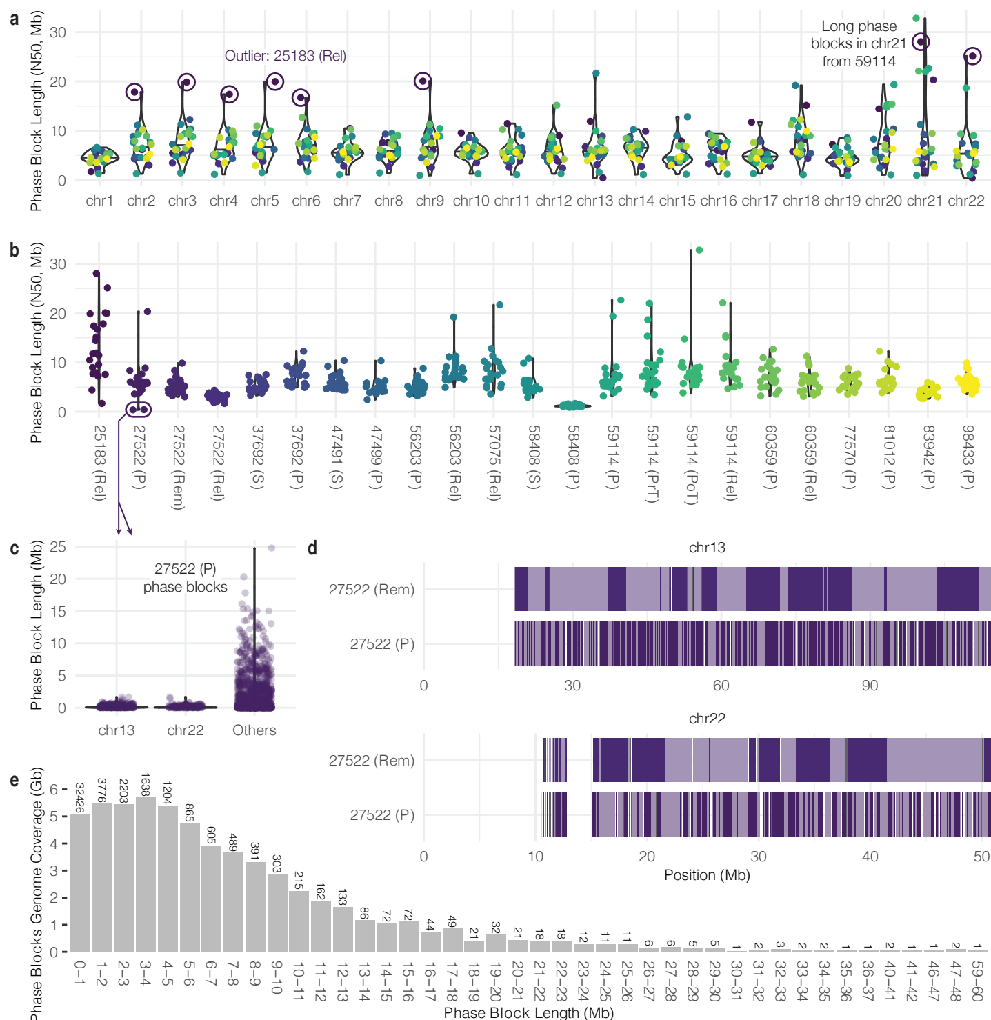
Supplementary Figure 2. Phase block length distribution. a. Phase block length by chromosome across all samples. Outlier phase blocks from sample 25183 (Rel) circled. Violin plots defined as: center line, median; violin limits, minimum and maximum values; points, every observation. b. Phase block length per sample across all chromosomes. c. Phase block lengths of chr13, chr22, and others from 27522 (P). Phase blocks less than 1 kb filtered out for plotting. d. Chr13 and chr22 phase block boundaries from 27522 (P) and 27522 (Rem). Alternating dark and light boxes indicate adjacent phase blocks. e. Total phase block genome coverage from all samples combined, grouped by phase block length.
