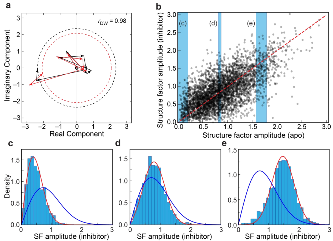
Figure 1: The double-Wilson model. a) In the double-Wilson model, the structure factors of related structures (black and red) are built up from pairs of random contributions (arrows) with correlation r_{DW} between their real components and likewise between their imaginary components. The experimentally observed amplitudes of the structure factors are described by the radii of the dashed circles. b) Scatter plot for structure factor amplitudes for isomorphous PTP-1B datasets for apo and inhibitor-bound forms (for a random subset of Miller indices). Blue slices indicate data points for which histograms are shown in panels c-e. c-e) Histograms for slices through panel b are better approximated by the Rice distributions (red) parametrized by a global r_{DW} (here 0.85) than by the unconditional, univariate Wilson distribution (blue).
