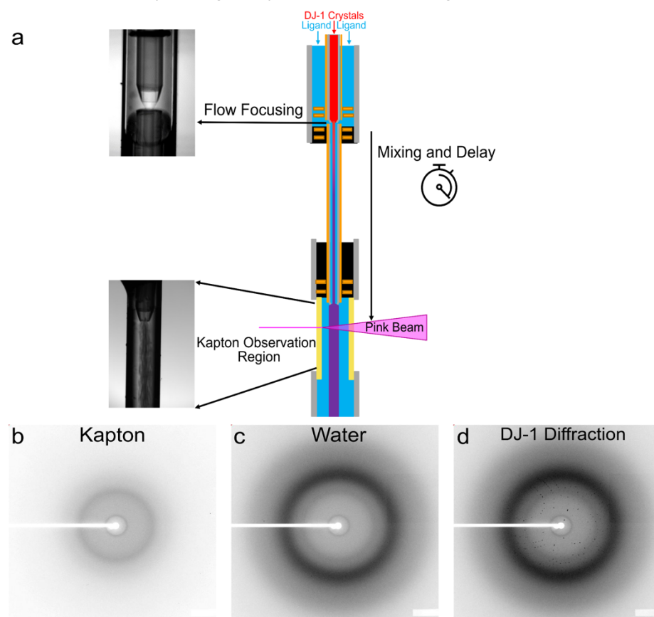
Figure 2: Flow-focused mixing injector for synchrotron MISC applications. Panel (a) shows the flow-focused diffusive mixer is constructed out of concentric capillaries and then coupled directly to a Kapton observation region. The crystal stream (red) is flow-focused by an external ligand stream (blue) to facilitate rapid diffusion of the ligand for reaction initiation. The fully mixed sample (purple) continues to flow and age until a desired timepoint is achieved. Flowrates and the position of the X-ray beam relative to the tip of the mixer can be modified to reach different timepoints. Background scattering from the empty (dry) Kapton tubing (panel (b)), background scattering from water flowing through the Kapton tubing (panel (c)), and representative diffraction pattern from a DJ-1 microcrystal while flowing through the Kapton tubing (panel (d)). Diffraction spots are clearly visible above the background scatter.
