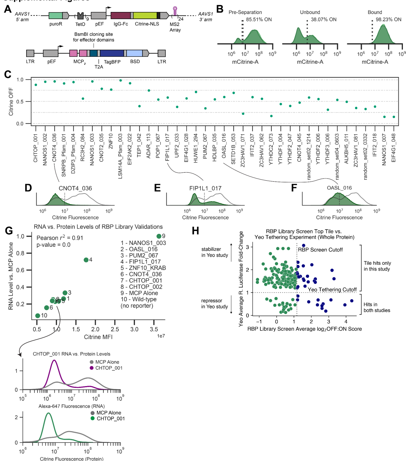
Figure S1. RBP library screen details, related to Figure 1. (A) Full construct schematic of the RNA recruitment reporter integrated into the AAVS1 safe harbor locus in the first intron of the PPP1R12C gene (top) and MCP-fusion vector for pooled domain cloning (bottom). puroR = puromycin resistance, TetO = tetracycline
