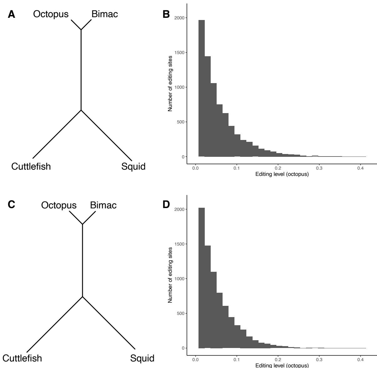
Figure S5: (A) Neighbor-joining tree of four coleoid species based on simulated neutral editing levels. (B) Distribution of neutral editing levels in the octopus. (C) Neighbor-joining tree of four coleoid species based on simulated deleterious editing levels. (D) Distribution of deleterious editing levels in the octopus.
