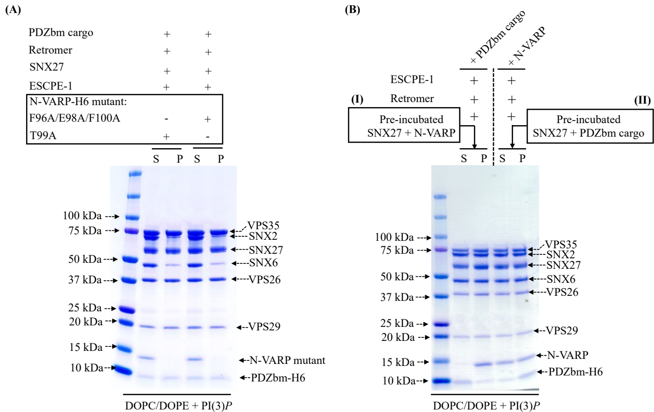
Figure 6. The VARP N-terminus is sufficient to recruit an endosomal supercomplex to membranes in vitro .
