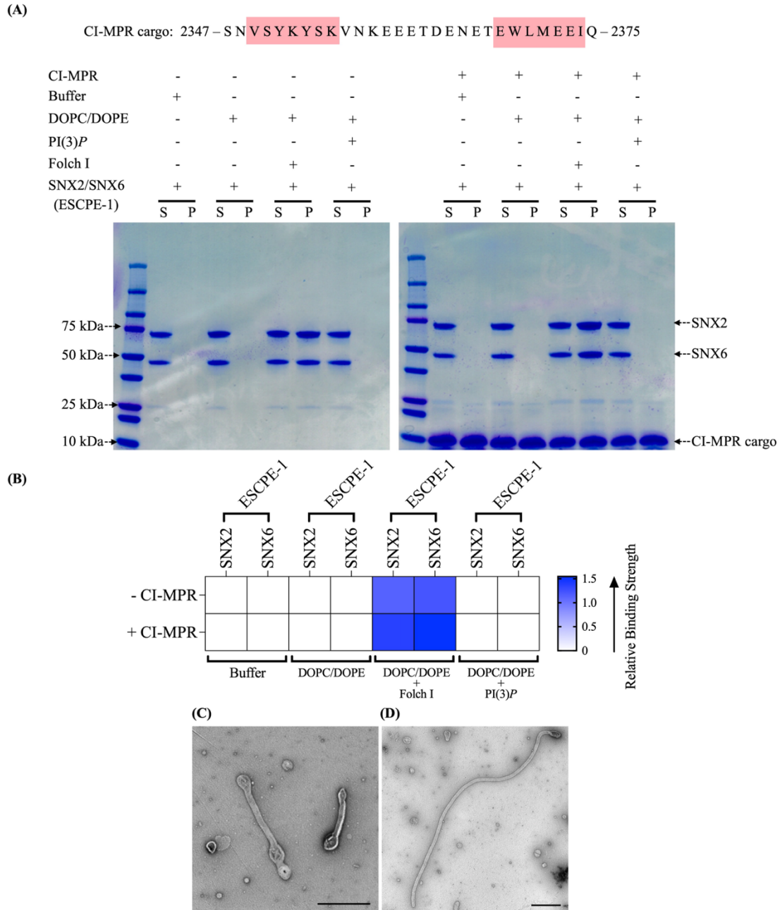
Figure S8. Membrane binding and tubulation properties of ESCPE-1 differ from those of SNX27/
