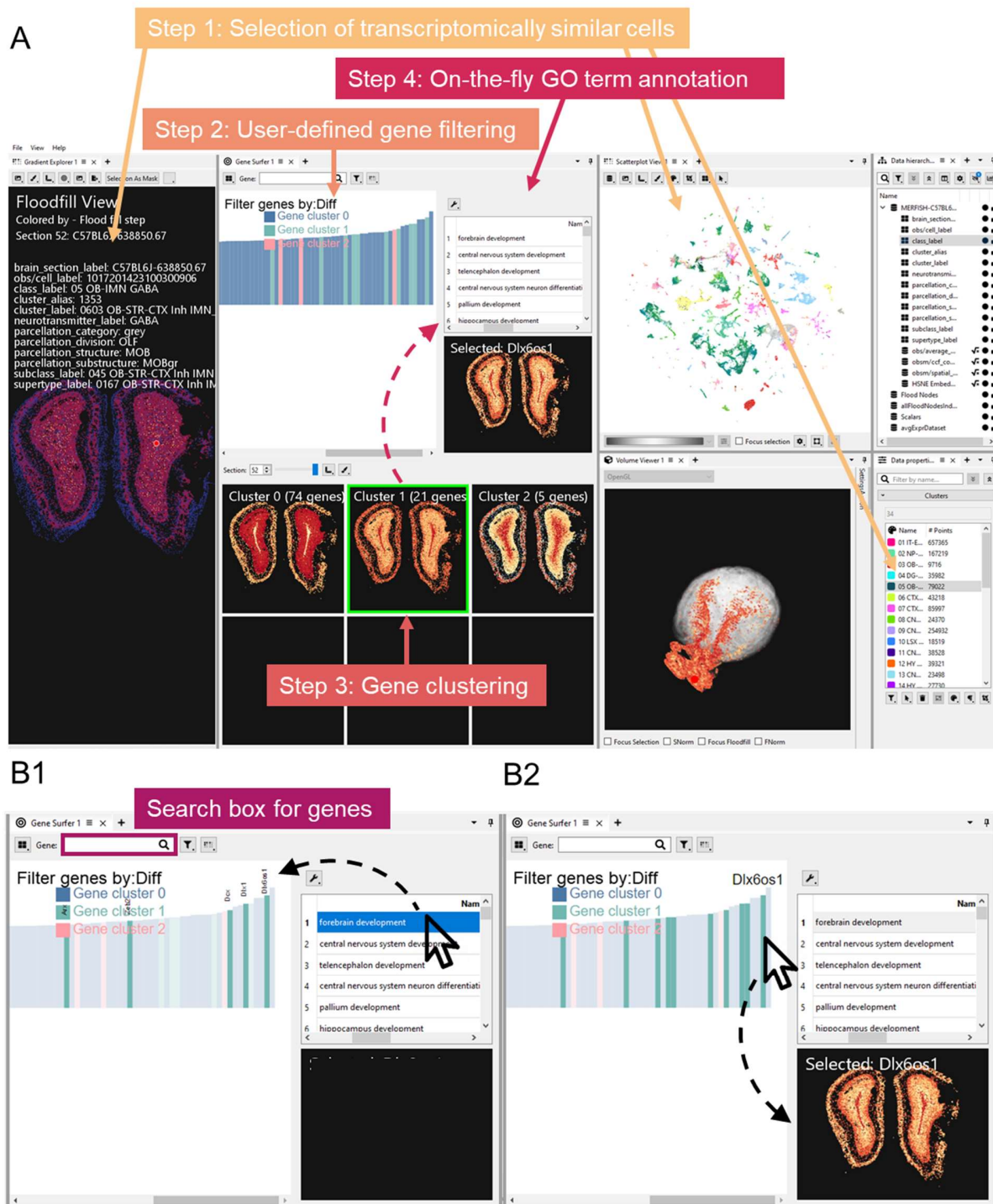
Figure 6. GeneSurfer interface and interaction loop. A. Screenshot of the interface of GeneSurfer with SpaceWalker. B1. When the user selects a GO term from the table, associated
