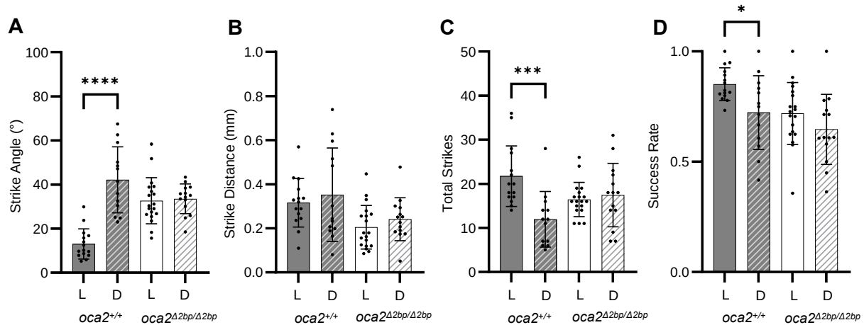
Figure 2 – oca2 mutant surface fish do not alter their strike dynamics in the dark. (A) Average strike angles of wild-type ( oca2 +/+ ) oca2 Δ2bp/Δ2bp surface fish in light and dark conditions. Welch's t test: oca2 +/+ , light, (n = 15) and dark (n = 13), p<0.0001. t test: oca2 Δ2bp/Δ2bp , light (n = 19) and dark (n = 14), p = 0.7862. (B) Average strike distances of wild-type and oca2 Δ2bp/Δ2bp surface fish in light and dark conditions. Welch's t test: oca2 +/+ , light, (n = 15) and dark (n = 13), p = 0.5856. t test: oca2 Δ2bp/Δ2bp , light (n = 19) and dark (n = 14), p = 0.3007. (C) Total number of strikes in wild-type and oca2 Δ2bp/Δ2bp surface fish in light and dark conditions. Mann-Whitney U test: oca2 +/+ , light, (n = 15) and dark (n = 13), p = 0.0001. Welch's t test: oca2 Δ2bp/Δ2bp , light (n = 19) and dark (n = 14), p = 0.6401. (D) Success rates of wild-type and oca2 Δ2bp/Δ2bp surface fish in light and dark conditions. Welch's t test: oca2 +/+ , light, (n = 15) and dark (n = 13), p = 0.0208. t test: oca2 Δ2bp/Δ2bp , light (n = 19) and dark (n = 14), p = 0.1804. All error bars are standard error of the mean. *p<0.05, **p<0.01, ***p<0.001, ****p<0.0001
