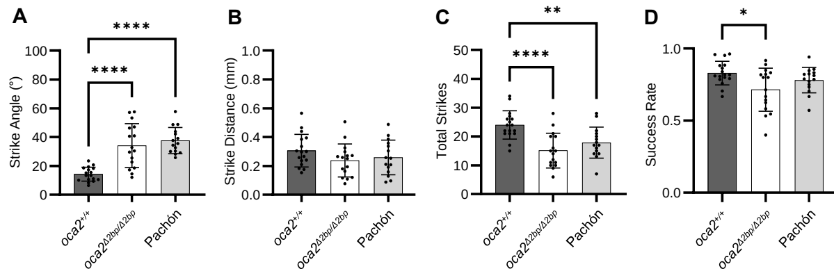
Figure 1 – oca2 mutant surface fish exhibit altered strike dynamics in the light. (A) Average strike angles of wild-type ( oca2 +/+ ) surface fish (n = 17), oca2 Δ2bp/Δ2bp surface fish (n = 16), and Pachón cavefish (n = 15). One way ANOVA, F(2, 45) = 23.30, p < 0.0001. Tukey's multiple comparisons test: oca2 +/+ vs oca2 Δ2bp/Δ2bp surface fish (Adjusted p < 0.0001), oca2 +/+ surface vs Pachón (Adjusted p < 0.0001), oca2 Δ2bp/Δ2bp vs Pachón (Adjusted p = 0.6398). (B) Average strike distances of oca2 +/+ surface fish (n = 17), oca2 Δ2bp/Δ2bp surface fish (n = 16), and Pachón cavefish (n = 15). One way ANOVA, F(2, 45) = 1.521, p = 0.2296. (C) Total number of strikes for oca2 +/+ surface fish (n = 17), oca2 Δ2bp/Δ2bp surface fish (n = 16), and Pachón cavefish (n = 15). One way ANOVA, F(2, 45) = 11.54, p < 0.0001. Tukey's multiple comparisons test: oca2 +/+ vs oca2 Δ2bp/Δ2bp surface fish (Adjusted p < 0.0001), oca2 +/+ surface fish vs Pachón (Adjusted p = 0.0074), oca2 Δ2bp/Δ2bp vs Pachón (Adjusted p = 0.3488). (D) Success rates of wild-type surface fish (n = 17), oca2 Δ2bp/Δ2bp surface fish (n = 16), and Pachón cavefish (n = 15). One way ANOVA, F(2, 45) = 4.445, p = 0.0173. Tukey's multiple comparisons test: oca2 +/+ vs oca2 Δ2bp/Δ2bp surface fish (Adjusted p = 0.0128), oca2 +/+ surface fish vs Pachón (Adjusted p = 0.4285), oca2 Δ2bp/Δ2bp vs Pachón (Adjusted p = 0.2363). All error bars are standard error of the mean. *p < 0.05, **p < 0.01, ***p < 0.001, ****p < 0.0001.
