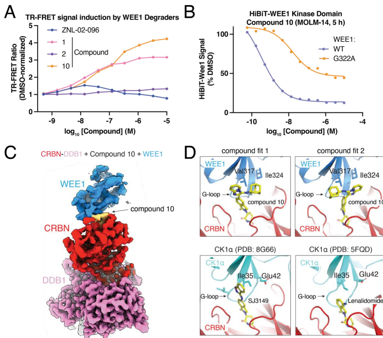
Figure 4. Structural characterization of WEE1 recruitment to CRBN facilitated by compound 10 . (A) Evaluation of TR-FRET signal induced by the hit compounds at a range of concentrations. (B) Mutation of the G-loop glycine leads to rescue of a HiBiT-WEE1 kinase domain degradation by compound 10 . (C) Density map of the DDB1-CRBN-compound 10 -WEE1 complex visualized by Cryo-EM (left) and magnified WEE1-CRBN interaction region with two possible compound binding modes (right). (D) Comparison of the binding modes of compound 10 and SJ3149 in the CRBN-kinase interaction pocket.
