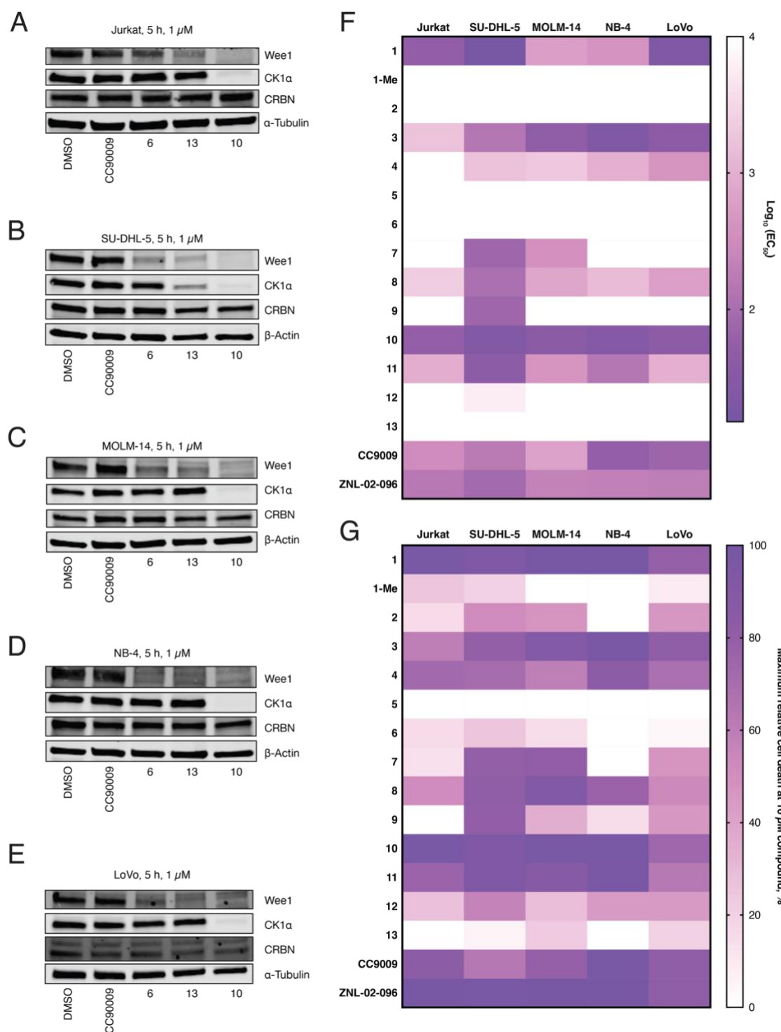
Figure 5. Characterization of the HRZ-1 scaffold derivatives CK1 \alpha /WEE1 degradation and anti-proliferative effect in a range of cancer cell lines. (A-E) Western blots showing consistent and preferential degradation of WEE1 by selective degraders 6 and 13 . CC90009 and Compound 10 were used as negative and positive controls, respectively. (F, G) Heat maps demonstrating effect of compounds 1-14 on the cancer cells viability using \text{EC}_{50} (compound concentration leading to half-maximal cell death) and the maximum relative cell death achieved at 10 \mu M treatment.
