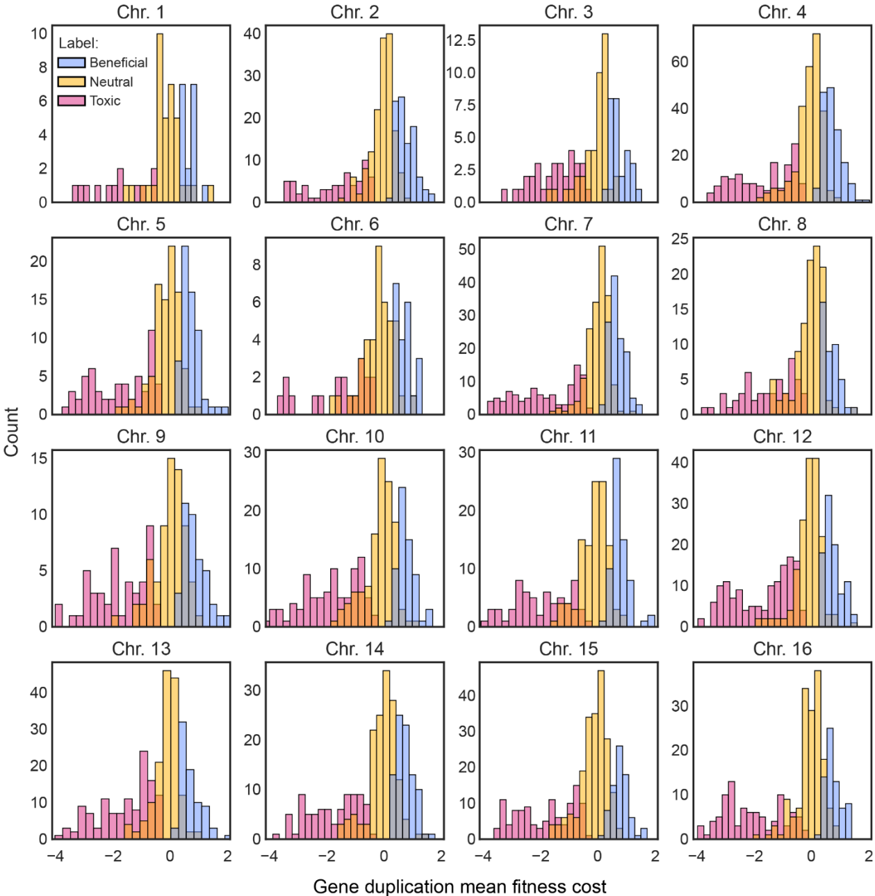
Figure S1. Distribution of gene fitness costs across each chromosome. Histogram of log2 fitness scores for single-gene duplications encoded on each chromosome, in each category, according to the key.
