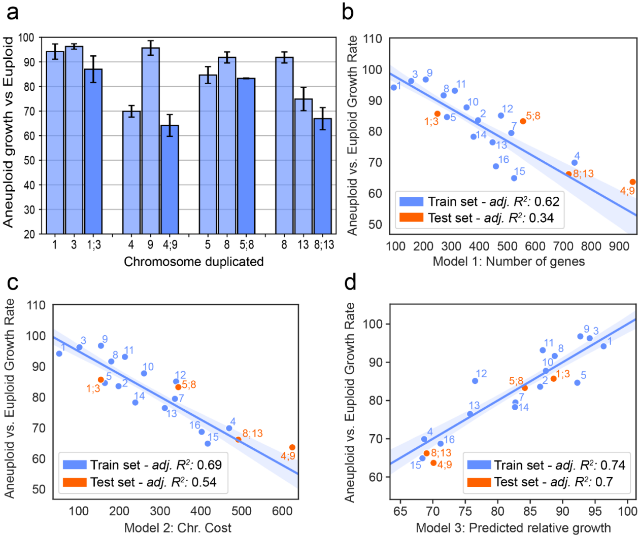
Figure S2. Model validation on dual-chromosome duplication strains. (A) Relative growth rates of strains with single- and dual-chromosome amplifications. (B-D) The explanatory power for dual aneuploids (orange points) is listed using the respective model trained against single aneuploids. Chromosome duplications are indicated by their number on the plots.
