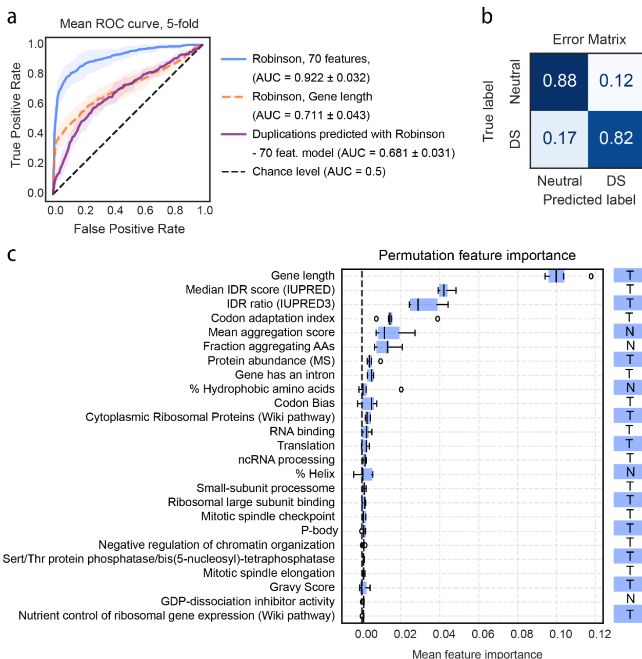
Figure 6. Model predictions applied to Robinson et al. 2-micron over-expression dataset. (A) As shown in Figure 5 but using the top 70 identified features applied to 400 commonly deleterious genes versus 1,657 commonly neutral genes based on Robinson et al. data 59 (blue curve). Robinson data fit only with gene length (dashed line), or gene-duplication data from this study (“Duplications”, purple curve) fitted with the model trained on Robinson data. (B) Error matrix for Robinson et al. model as described in Figure 5. (C) Mean and standard deviation of the feature importance measured with respect to ROC-AUC gain (see Methods) for Robinson’s model with the top 25 features, as shown in Figure 5. A complete report of the permutation feature importance for all 70 features of the model is available in Fig.6C supplemental table.
