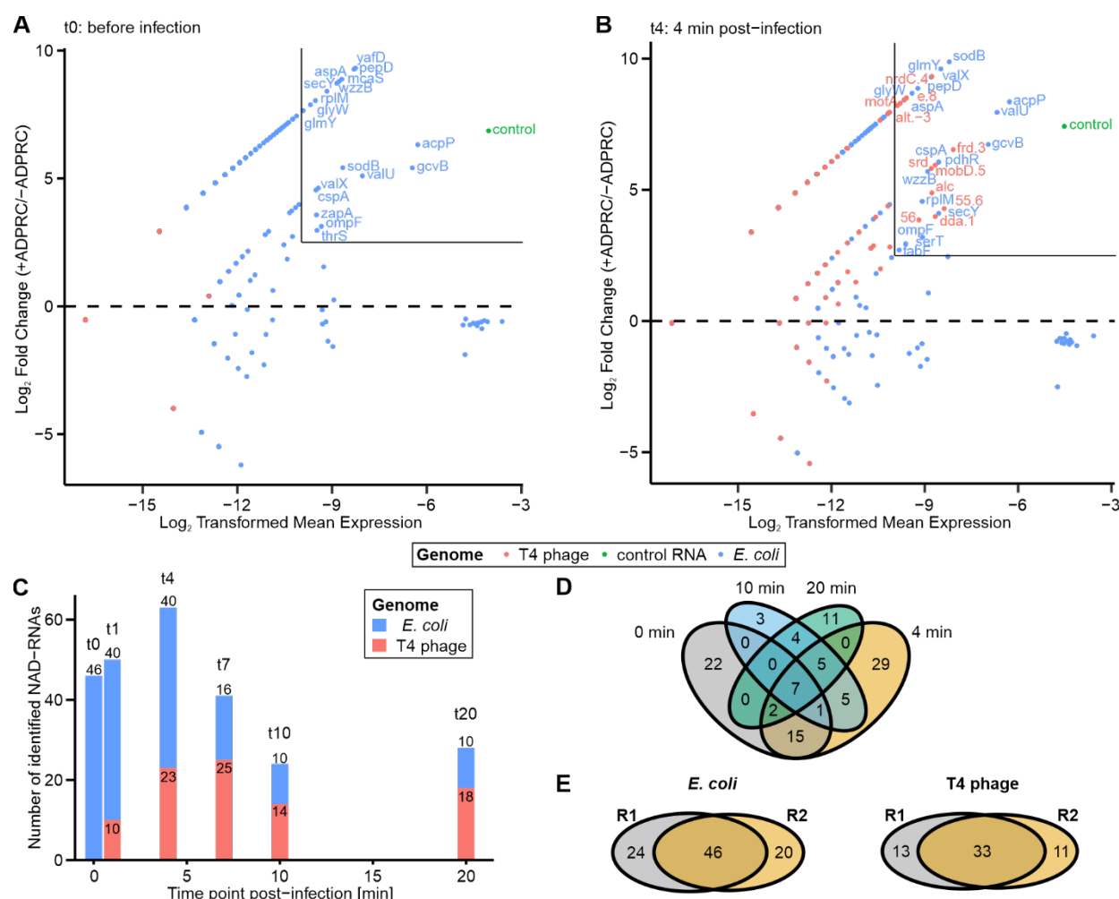
Figure 2: Identification of NAD-RNAs using time-resolved dual NAD captureSeq.
