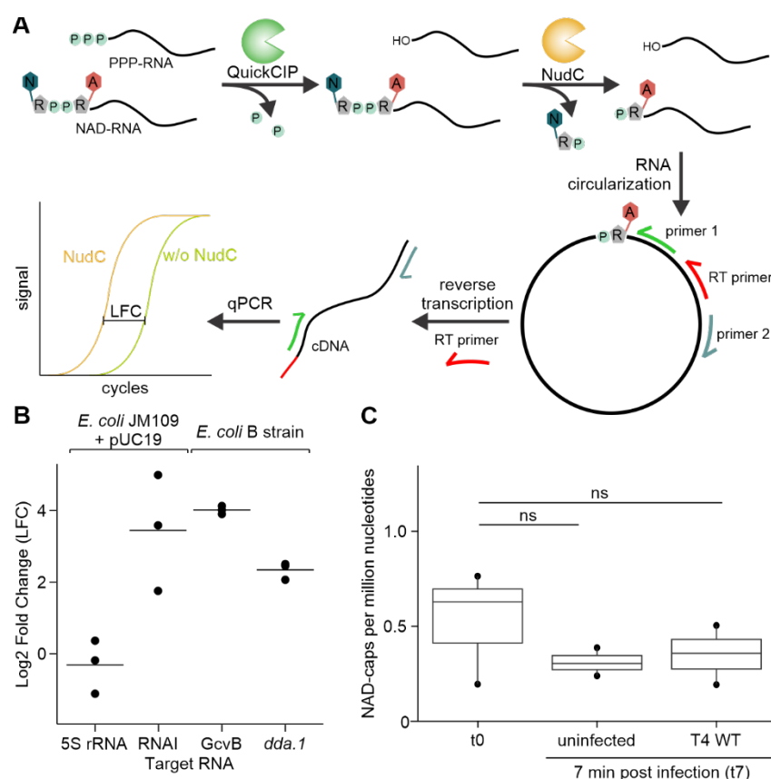
Figure 3: Validation of NAD-RNAs via a circNC-like assay and LC-MS.
