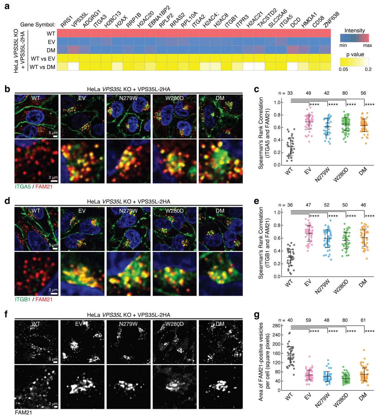
Fig. 4 Disrupting the SNX17-Retriver interaction impairs PM homeostasis
