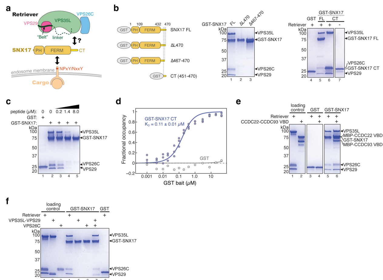
Fig. 1 SNX17 uses its C-terminal tail to bind Retriever
