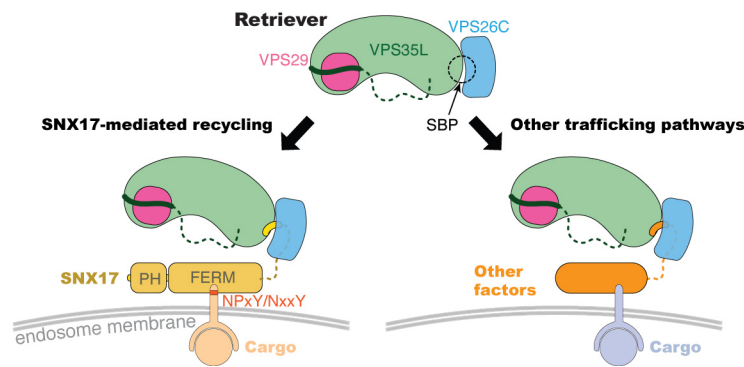
Fig. 6 Schematic of Retriever-mediated endosomal recycling.
