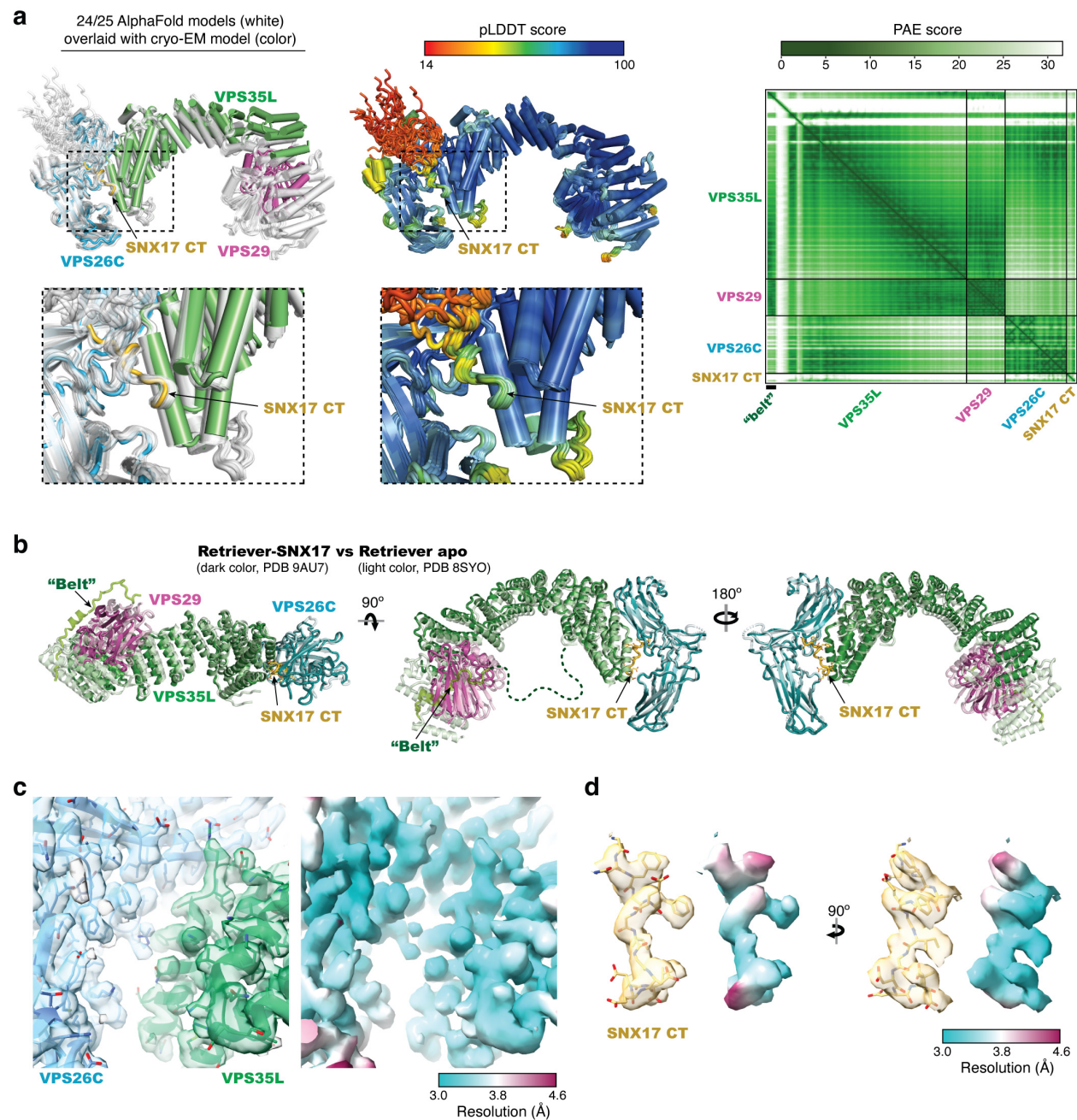
Extended Data Fig. 3 Overall structure comparison and local map quality.
