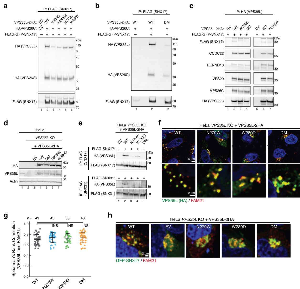
Fig. 3 Disrupting the SBP impairs SNX17 and SNX31 binding in cells
