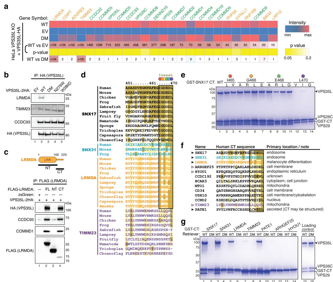
Fig. 5 Interactome analysis reveals other Retriever ligands with an acidic CT tail.
