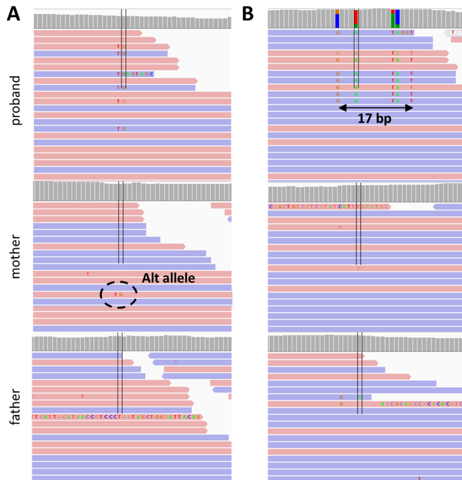
Figure 2. Main indicators of false-positive variants, which are removed after force-calling and second QC. A. Reads containing alternative alleles in parental read alignments. B. Accumulation of de novo SNVs in a relatively restricted genomic area.
