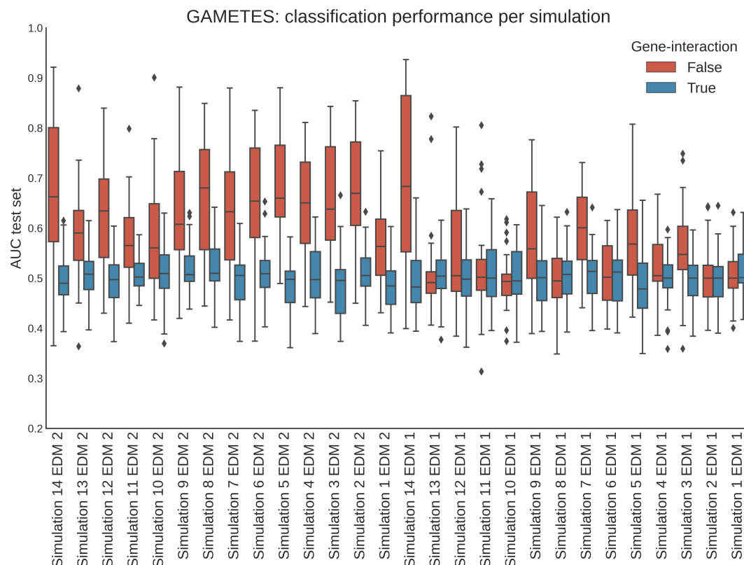
Fig. 6. Boxplot of the predictive performance in area under the curve for the GenNet neural networks on the different Gametes simulations for the simulations with the interacting pair in the same gene and simulations with the interacting variants in a different gene (gene-interaction). See Supplementary Table 2 for the simulation specifications
