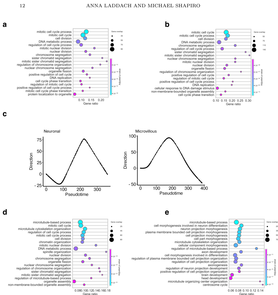
FIGURE 7. a ) Dot plot showing GO terms overrepresented among transiently upregulated genes at DP2 for the neuronal trajectory (the intersection of the top 5% up-regulated genes in the DP1-DP2 direction with the top 5% of downregulated genes in the DP2-Neurons direction). Dot size indicates the overlap for each term, and gene ratio indicates the fraction of genes in each term. b ) As in a) for the top 5% of genes associated with PC2. c ) Line graphs showing the progress of smoothed trajectories projected onto PC2. d ) As in a) for the top 5% of genes associated with the DP1-neuron directionality. e ) As in a) for the top 5% of genes associated with the DP1-neuron directionality omitting PC2.
