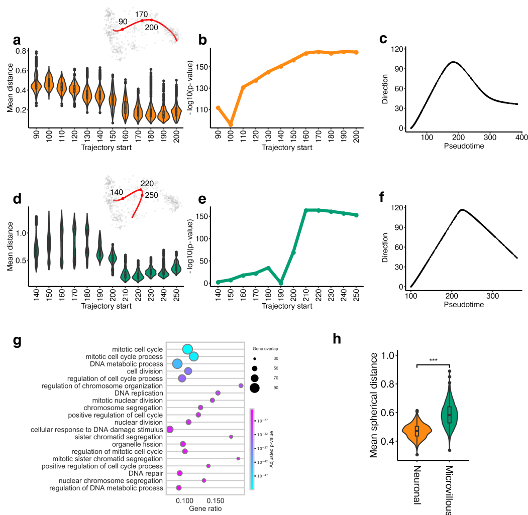
FIGURE 6. a ) Violin plots indicating the mean spherical distance for the neuronal trajectory (first 3 PCs) starting from successively later points in pseudotime, as DP2 is approached (value 170 on the neuronal trajectory shown in the top right inset). b ) Line graph indicating the -\log_{10}(p\text{-value}) for the significance of directionality for the neuronal trajectory (first 3 PCs) relative to random trajectories, starting from successively later points in pseudotime. d ) Line graph showing progress of the smoothed neuronal trajectory (available in 5 PCs) projected onto the DP1-DP2 directionality. d ) Violin plots indicating the mean spherical distance for the microvillous trajectory (first 3 PCs) starting from successively later points in pseudotime, as DP2 is approached (value 220 on the microvillous trajectory shown in the top right inset). e ) Line graph indicating the -\log_{10}(p\text{-value}) for the significance of directionality for the microvillous trajectory (first 3 PCs) relative to random trajectories, starting from successively later points in pseudotime. f ) Line graph showing progress of the smoothed microvillous trajectory (available in 5 PCs) projected onto the DP1-DP2 directionality. g ) Dot plot showing GO terms overrepresented among the top 5 % of transiently upregulated genes at DP2 for the microvillous trajectory. Dot size indicates the overlap for each term, and gene ratio indicates the fraction of genes in each term. h ) Violin plots indicating the mean spherical distance of the neuronal (orange) and microvillous (green) trajectories from DP1 onwards using 1000 random paths from each trajectory and PCs 1, 3-10 (omitting PC2).
