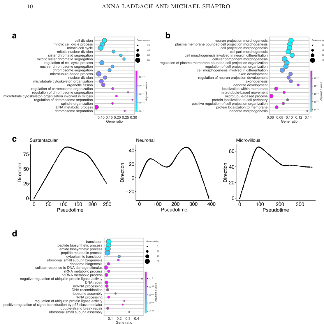
FIGURE 5. a ) Dot plot showing GO terms overrepresented among the top 5 % of genes associated with the HBC-neuron directionality. Dot size indicates the overlap for each term, and gene ratio indicates the fraction of genes in each term. b ) As in a ) for genes associated with the DP2-neuron directionality. c ) Line graphs showing the progress of smoothed trajectories projected onto PC4. d ) As in a ) for the top 5% of genes associated with PC4.
