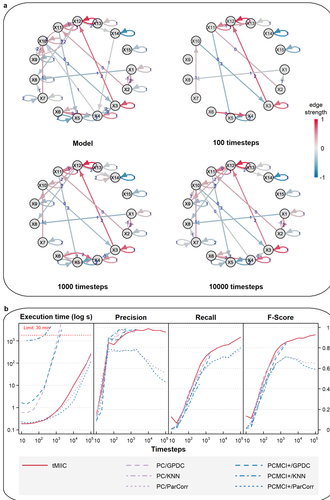
Supplementary Fig. 1. Benchmark assessment of CausalXtract's causal discovery module (tMIIC) using generated time series datasets.
