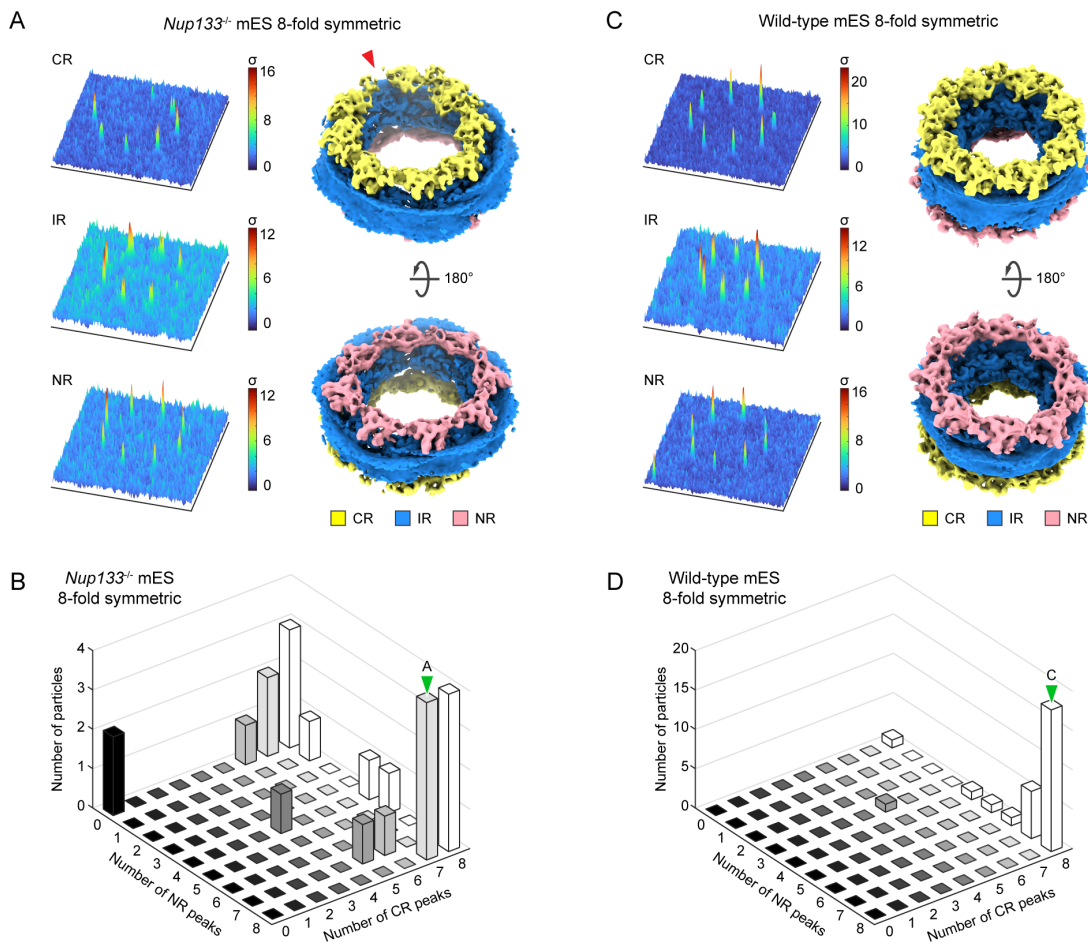
Figure 5: The 8-fold symmetric NPCs in the Nup133 -/- mES cells more frequently possess incomplete CR and NR architectures in comparison to the wild-type mES NPCs
