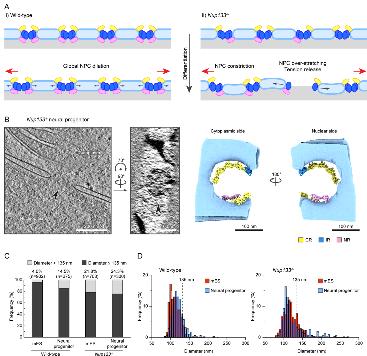
Figure 6: Over-stretched NPCs are present in the Nup133 -/- neural progenitor cells
