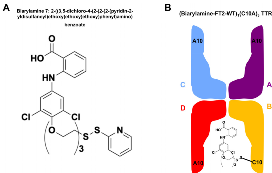
Supplementary Figure 16. TTR reaction with Biarylamine 7 ligand (2-((3,5-dichloro-4-(2-(2-(2-(pyridin-2-ylidisulfaneyl)ethoxy)ethoxy)ethoxy)phenyl)amino)benzoate) to afford the (biarylamine-FT 2 -WT) 1 (C10A) 3 TTR conjugate. (A) Chemical structure of Biarylamine 7 ligand. (B) Cartoon depiction of the (biarylamine-FT 2 -WT) 1 (C10A) 3 TTR adduct, covalently linked through subunit B.
