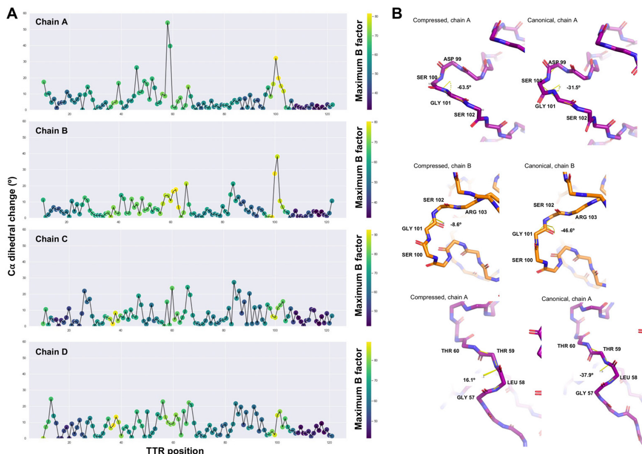
Supplementary Figure 29. Backbone angle changes between the compressed and canonical (Stilbene) 2 -TTR conformations. (A) Per-position C\alpha dihedral changes, colored by the highest B-factor value between the two compared models. (B) Backbone-only representation of positions with the highest dihedral angle changes: Ser100 from chain A, Gly101 from chain B, and Leu58 from chain A. The C\alpha dihedral angle values are shown.
