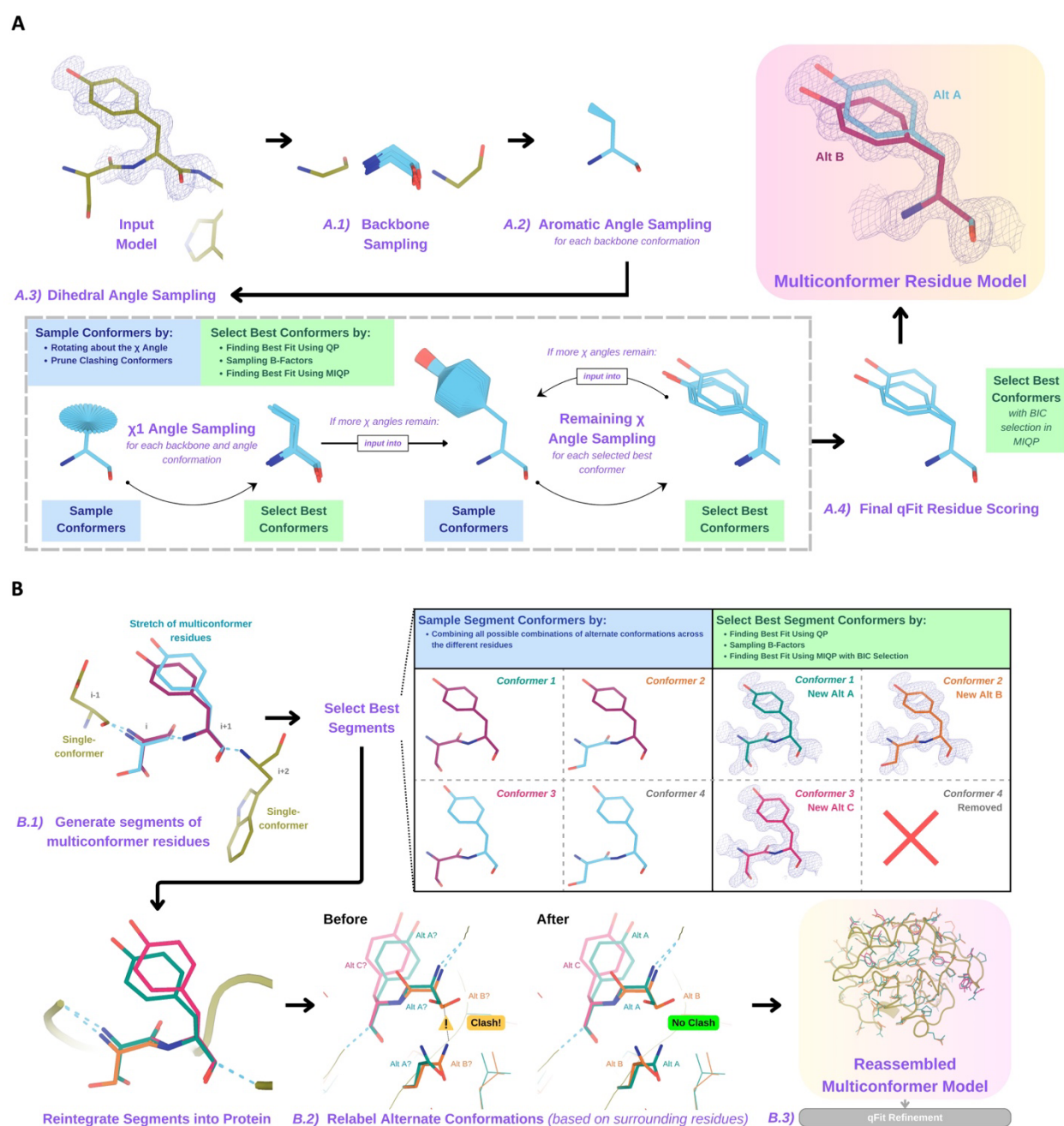
Figure 1. Programmatic flow of qFit protein algorithm.
