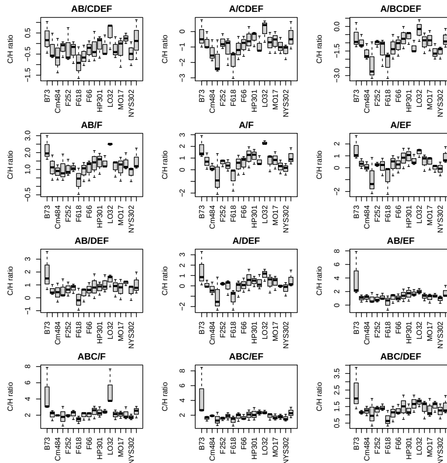
Fig. 6. Differences between lines according to the grouping choices Barplot representation of the variable CRatio for each maize inbred line. Grouping models have been range according to their anova R2 value.
