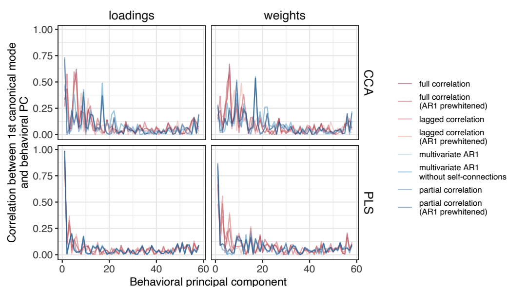
Figure 10: Similarity between first behavioral principal component and loadings or weights, for both CCA and PLS. For PLS, the correlation between loadings or weights and the first PC was very high. For CCA, the correlation with the first PC was high for loadings but moderate for weights. The differences between the FC methods were generally small, but somewhat larger for CCA than for PLS.
