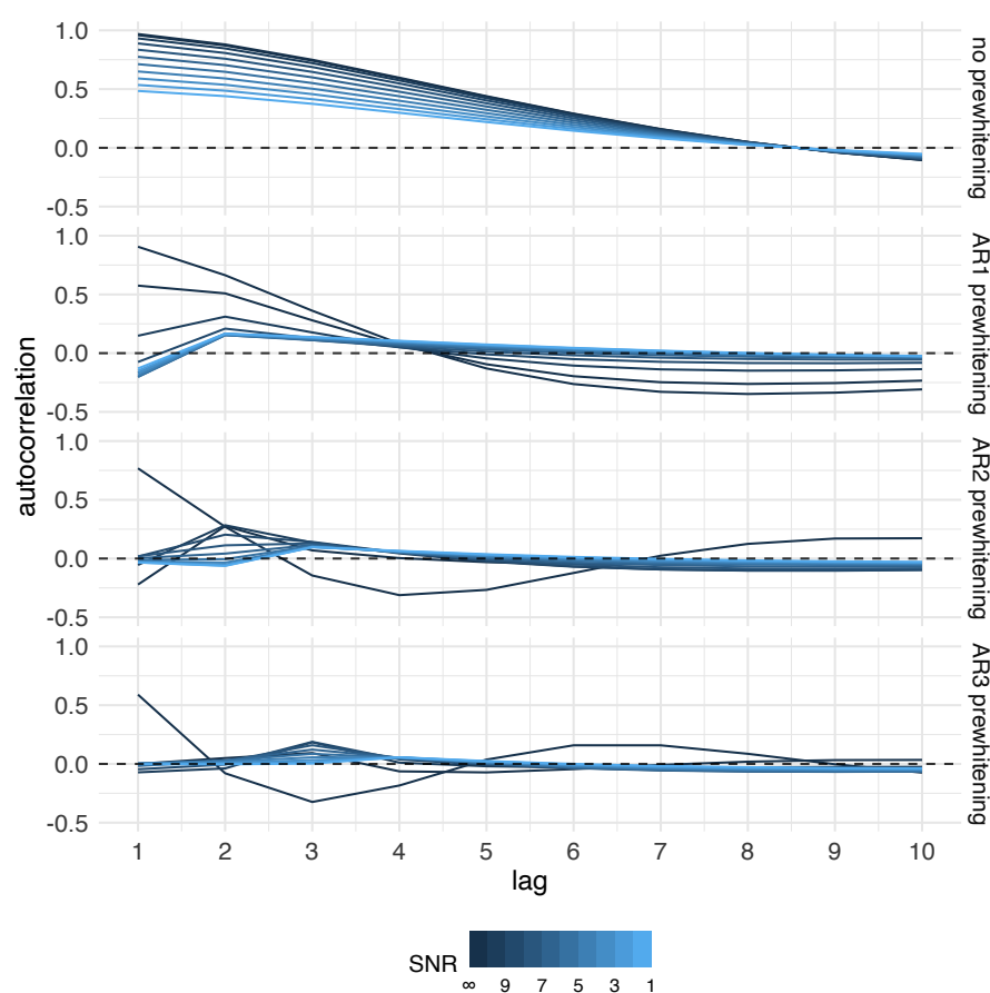
Figure S1: The autocorrelation function of simulated data as a function of prewhitening order and noise. The mean autocorrelation function was computed over all participants and regions. In general, noise and prewhitening reduced absolute autocorrelation. The shape of the autocorrelation function varied as a function of noise and prewhitening. In case without prewhitening, autocorrelation monotonically decreased and reached 0 at lag 8. After prewhitening, autocorrelation varied between positive and negative values, and this was most pronounced in cases without noise. The autocorrelation function was more similar to the experimental data in cases with low levels of noise.
