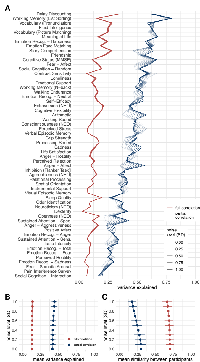
Figure 8: Results of variance component model for brain-behavior associations on data with added noise. FC was estimated using Pearson's/ full correlation and partial correlation after adding various levels of random Gaussian noise to experimental time series. A. Variance explained for individual traits estimated with different connectivity methods. Traits are ordered according to the mean variance explained across connectivity methods. B. Mean variance explained. Error bars represent jackknife standard deviation. C. Mean similarity between participants. Error bars represent standard deviation.
