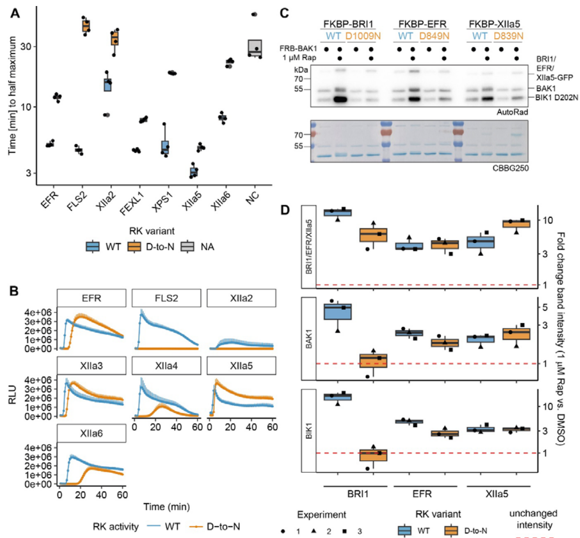
Figure 5 – Supplement 1: Xlla5 D839N exhibits largely Xlla5WT-like characteristics. A,B) Catalytic site mutation of Xlla5 exhibited the least delayed onset of oxidative burst. In A, quantification of the time to reach the half maximum of the oxidative burst is shown. The underlying data are the same as used for total oxidative burst in the main figure. In B, the actual oxidative burst curves are presented as average of six individual plants transiently expressing the indicated chimeric protein. Error bars represent standard error of the mean. C) A catalytic site mutation of Xlla5 did not negatively affect BIK1 trans-phosphorylation or BAK1 autophosphorylation. Experiments were performed as described in Figure 1. D) Quantification of band intensities on autoradiographs from three independent experiments are shown. BRI1 D1009N and EFR D849N displayed results similar to Figure 1B,C. In contrast to
