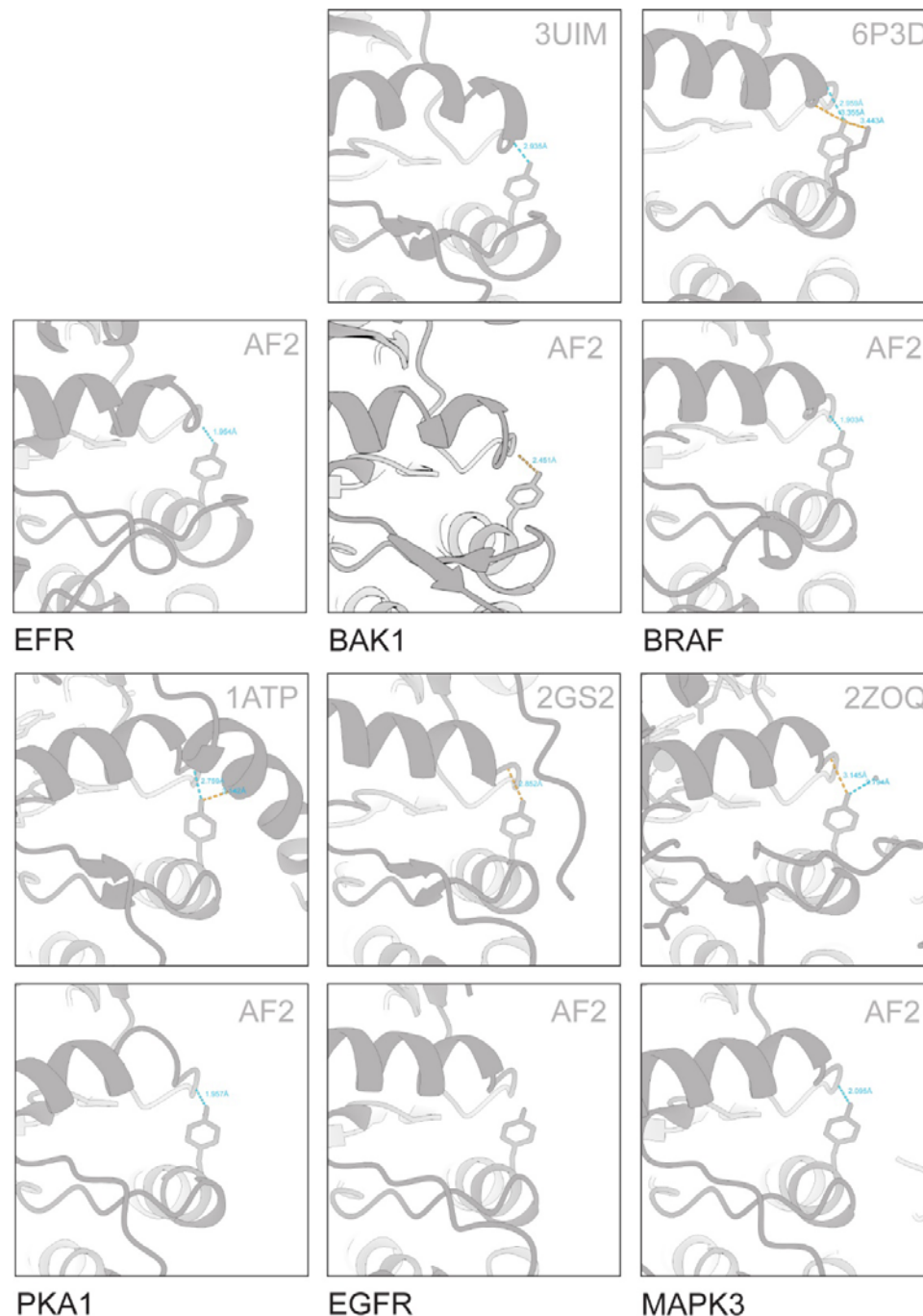
Figure 2 - Supplement 1: V6A-Tyr forms H-bonds with the \alpha C- \beta 4 loop in various predicted and solved structures. Solved structures were retrieved from PDB. AlphaFold2 models for kinases in their active conformation were retrieved from (Faizov and Dunbrack, 2023). BAK1 and EFR models were predicted by AlphaFold2, using the complete intracellular domain. H-bonds were predicted in ChimeraX and distances are indicated.
