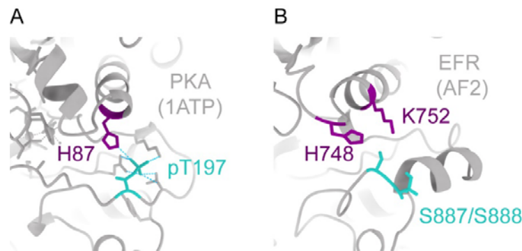
Figure 2 Supplement 3: EFR A-loop phosphorylation sites may coordinate with basic residues from the \beta 3 - \alpha C loop and \alpha C -helix. A) In PKA (1ATP), the A-loop phosphorylation on T197 coordinates with H87 from the \alpha C -helix. B) In EFR (AlphaFold2 (AF2) model), there are two basic residues extending downwards from \beta 3 - \alpha C loop (H748) and \alpha C -helix (K752) that may coordinate with A-loop phosphorylation on S887 or S888.
