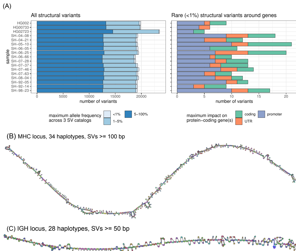
Figure 6. Structural variant landscape summary. (A) The number of structural variants across samples. In the left panel, structural variants were annotated with three SV catalogs (the gnomAD-SV database, a long-read-based SV catalog, and the HPRC v1.0 SV catalog). SVs are matched if they have at least 10% genomic overlap. SVs close to centromeres, telomeres, or within segmental duplications were removed. The colors highlight the maximum frequency across these catalogs, the lighter blue showing “rare” SVs (with an allele frequency below 1%) in the catalogs, or unmatched. SVs may be unmatched, either because they are novel or due to the difficulties in the database comparison. The right panel shows the number of rare structural variants in protein-coding genes, grouped by their impact on the gene structure. (B) MHC pangenome built from 28 brain and 6 cell line haplotypes, containing 640 nodes, SVs over 100bp are shown. (C) IGH pangenome built from 28 brain haplotypes containing 268 nodes. In contrast, cell lines are typically derived from B-cell lymphocytes and contain extensive somatic rearrangements in this locus.
