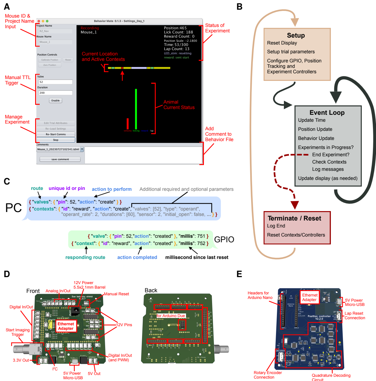
Figure 2. Details of UI function. (A) Screenshot of the UI. The interface provides a snapshot of the animal's current status (center) as well as cumulative information about the current experiment (upper-left). The control panel along the left side provide: Top . an input for a project name and mouse id, which control where the resulting behavior file will be saved (these boxes are disabled when an experiment is currently running), Middle . controls to trigger the GPIO to send a TTL pulse i.e. to issue a water reward or turn on an LED, and Bottom . controls to start/stop experiments as well as to load settings files. (B) Details of UI event loop. The UI is continuously executing an event loop on every update step which checks for messages, writes the behavior file and updates the display. (C) JSON formatted message passing. The PC sends and receives JSON formatted messages via UDP to active components of the system. Messages have a nested structure to allow for internal routing and subsequent actions to be taken. (D) Rendering of the GPIO circuit used. Left . JST headers connected to I/O pins and pull-down resistors to allow for easy connections with peripheral devices that can be activated by TTL pulses (both at 3.3V and 12V, depending on the pins used). Additionally, power connections and a BNC output trigger are provided. Right . This board attaches to an Arduino Due microcontroller. (E) Updates to the position have a dedicated circuit for decoding quadrature information and sending updates to the PC. Connections for a quadrature based rotary encoder, power, and Ethernet are provided. Additionally, an input for a "Lap Reset" sensor is provided and headers to interface with an Arduino Mini.
