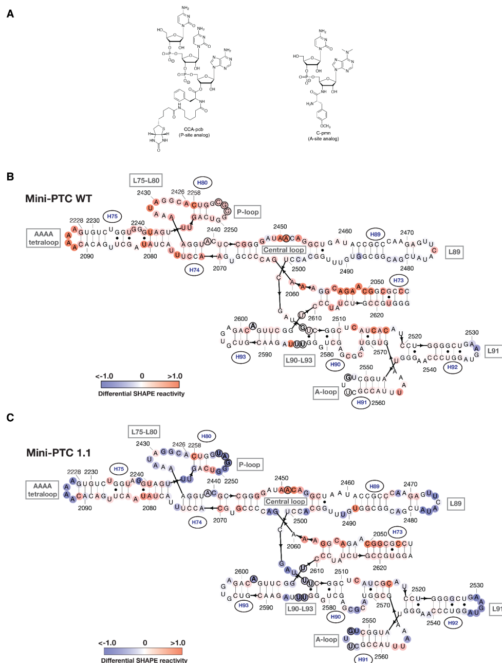
Figure 5. Mini-PTC 1.1 engages the ribosomal A- and P-site substrate mimics better than WT mini-PTC (A) Chemical structures of CCA-pcb (P-site analog) (left), and C-pmn (A-site analog) (Right). (B-C) Predicted secondary structure diagram showing differential SHAPE reactivities of WT mini-PTC (B) and mini-PTC 1.1 (C) in the presence of 100 \mu M CCA-pcb and 100 \mu M C-pmn. Differential SHAPE reactivities were represented on a blue-white-red spectrum, with blue indicating low changes, red indicating high changes, and white indicating no changes in SHAPE reactivity upon substrate binding. Previously identified 13 PTC residues that become protected upon binding A- or P-site tRNA substrates in the ribosome-tRNA complexes were indicated in circled residues. 5 of 13 residues in WT mini-PTC (B) and 12 of 13 residues in mini-PTC 1.1 (C) that become protected upon binding substrate mimics were highlighted as bold residues.
