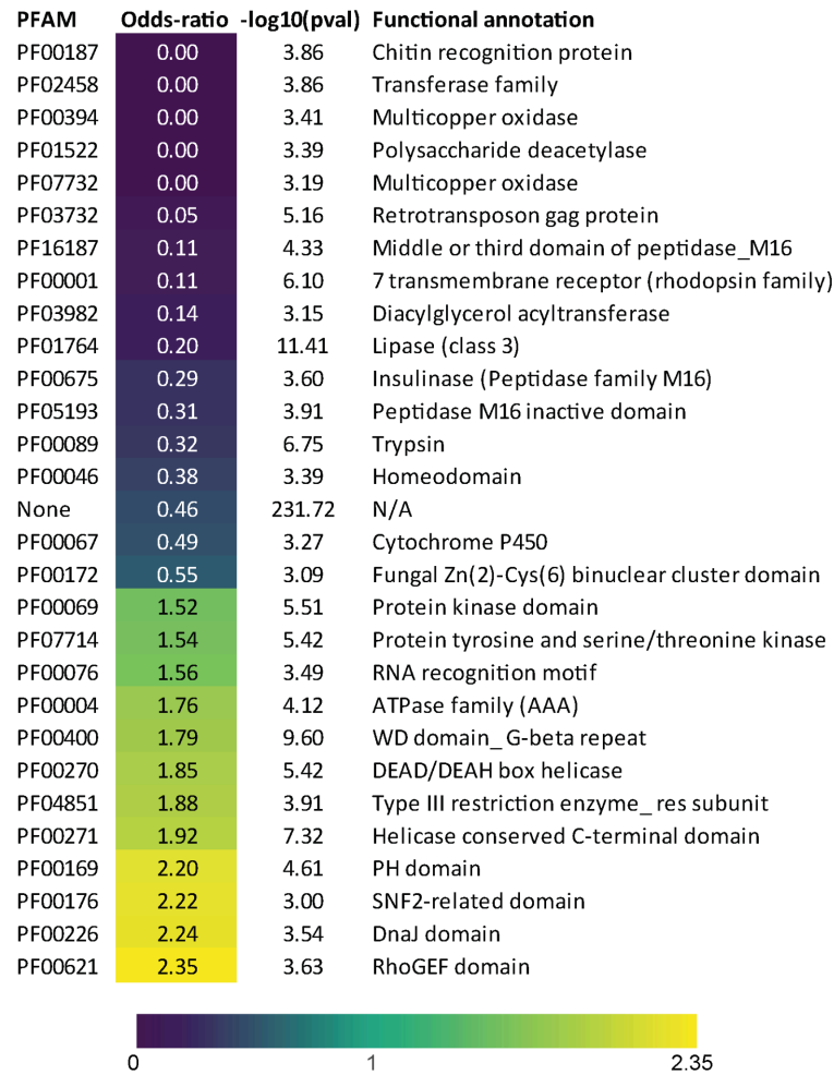
Figure 3-S3. E. muscae core OG Pfam enrichment. Enrichment among Pfam annotations for E. muscae genes belonging to core OG set. Odds-ratios are colored according to the scale bar below.
