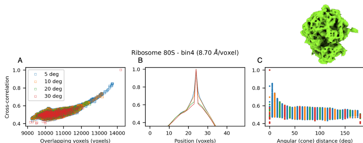
SI Fig. 4: Evaluation of increasing the number of orientations in template matching of ribosome 80S using the python tool for in silico evaluation. A, Cross-correlation as a function of the absolute number of overlapping voxels for all evaluated rotations. B, Cross-correlation as a function of the distance along the z-plane. C, Cross-correlation for all evaluated rotations as a function of the angular cone distance. With an increasing number of orientations (decreasing angular sampling), more rotations lead to a higher number of overlapping voxels and thus to a higher cross-correlation. This effect leads to a broadening of the peak in the middle panel.
