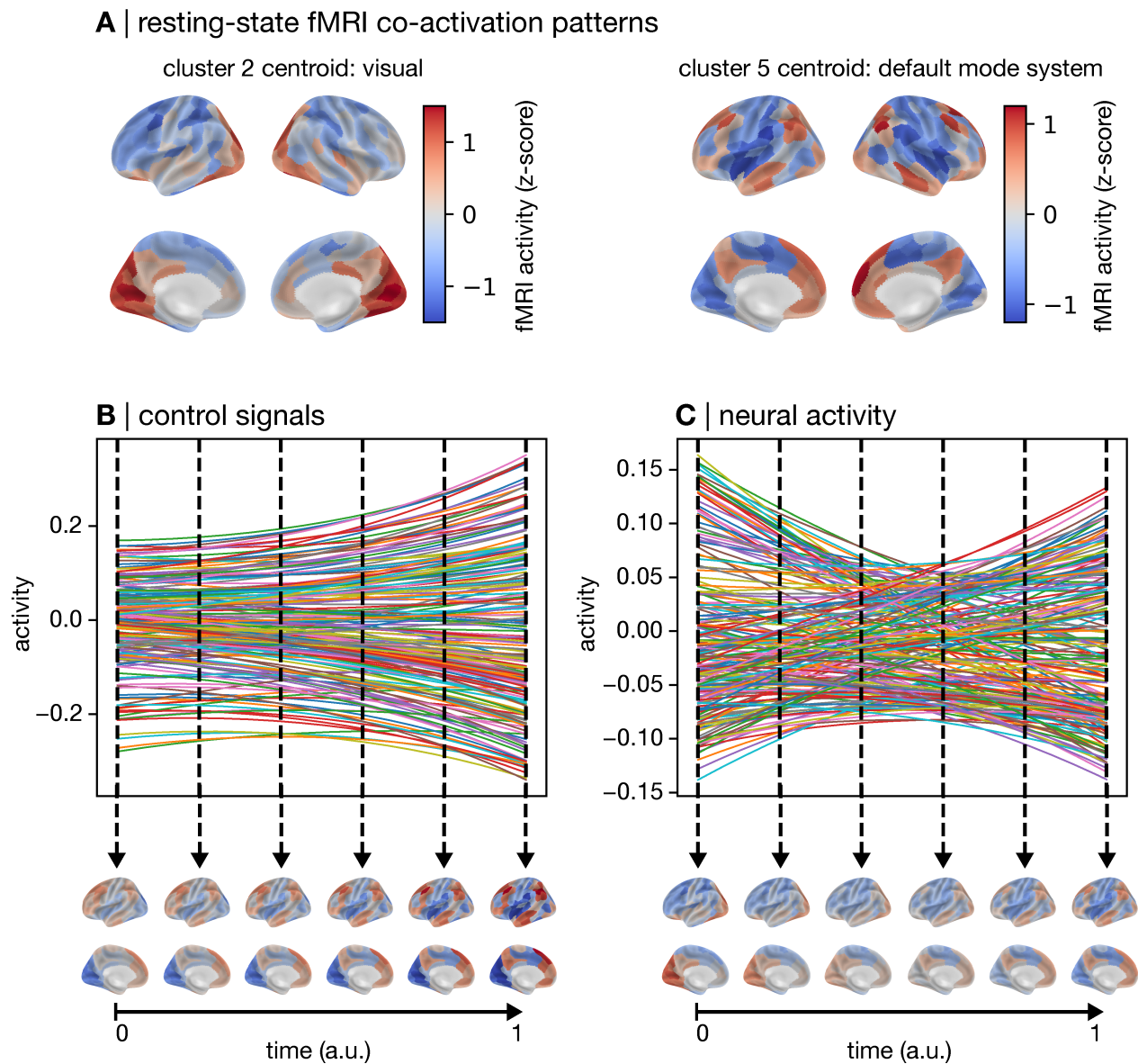
FIG. 6 Control signals and state trajectory for non-binary brain states derived from resting-state fMRI. We applied K-means clustering to resting-state fMRI time-series to extract patterns of co-activation. These patterns were used as non-binary brain states for network control theory (NCT) analysis. A , Resting-state fMRI clusters that represent visual system activity (left) and default mode activity (right). The control signals and the state trajectory were modeled by assigning the visual system to the initial state and the default mode system to the target state. B , Control signals visualized using line plots (top) and on the cortical surface for select time points (bottom). C , State trajectory (neural activity) visualized using line plots (top) and on the cortical surface for select time points (bottom).
