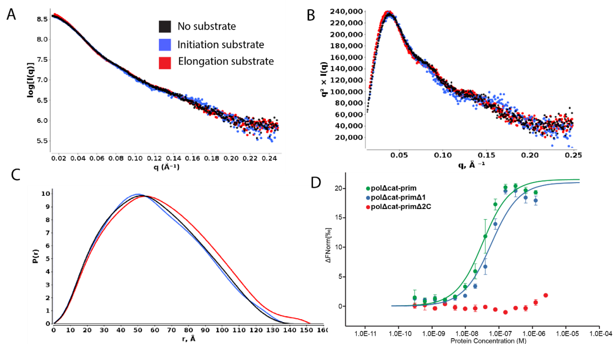
Figure 3. RNA elongation substrate engagement in solution. Comparison of SAXS data for free polΔcat-prim (black) and polΔcat-prim in the presence of an RNA elongation substrate (red), and substrate and co-factors required for initiation (blue): A) log 10 intensity plot; B) normalized Kratky plot; C) distance distribution. D) MST dose-response curve measuring RNA elongation substrate binding of polΔcat-prim (green), polΔcat-primΔ1 (blue), and polΔcat-primΔ2C (red).
