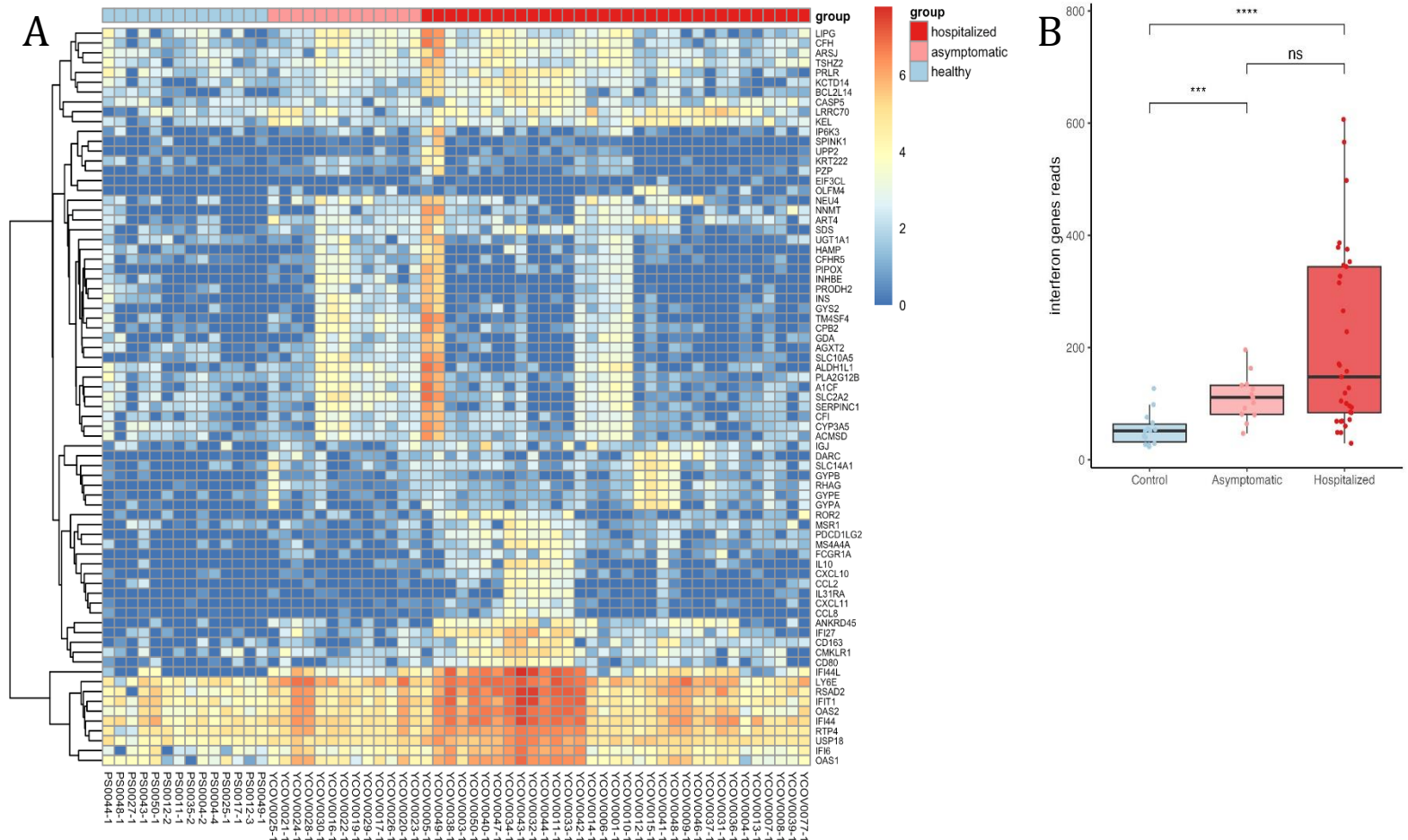
Figure 6: Chromatin immunoprecipitation of cell-free nucleosomes analysis of COVID-19 patients, asymptomatic and controls. (A) Unsupervised clustered heat map of the genes that are significantly elevated in the hospitalized COVID-19 patients, compared to controls. (B) reads of genes from a predefined interferon response gene set in the three groups.
