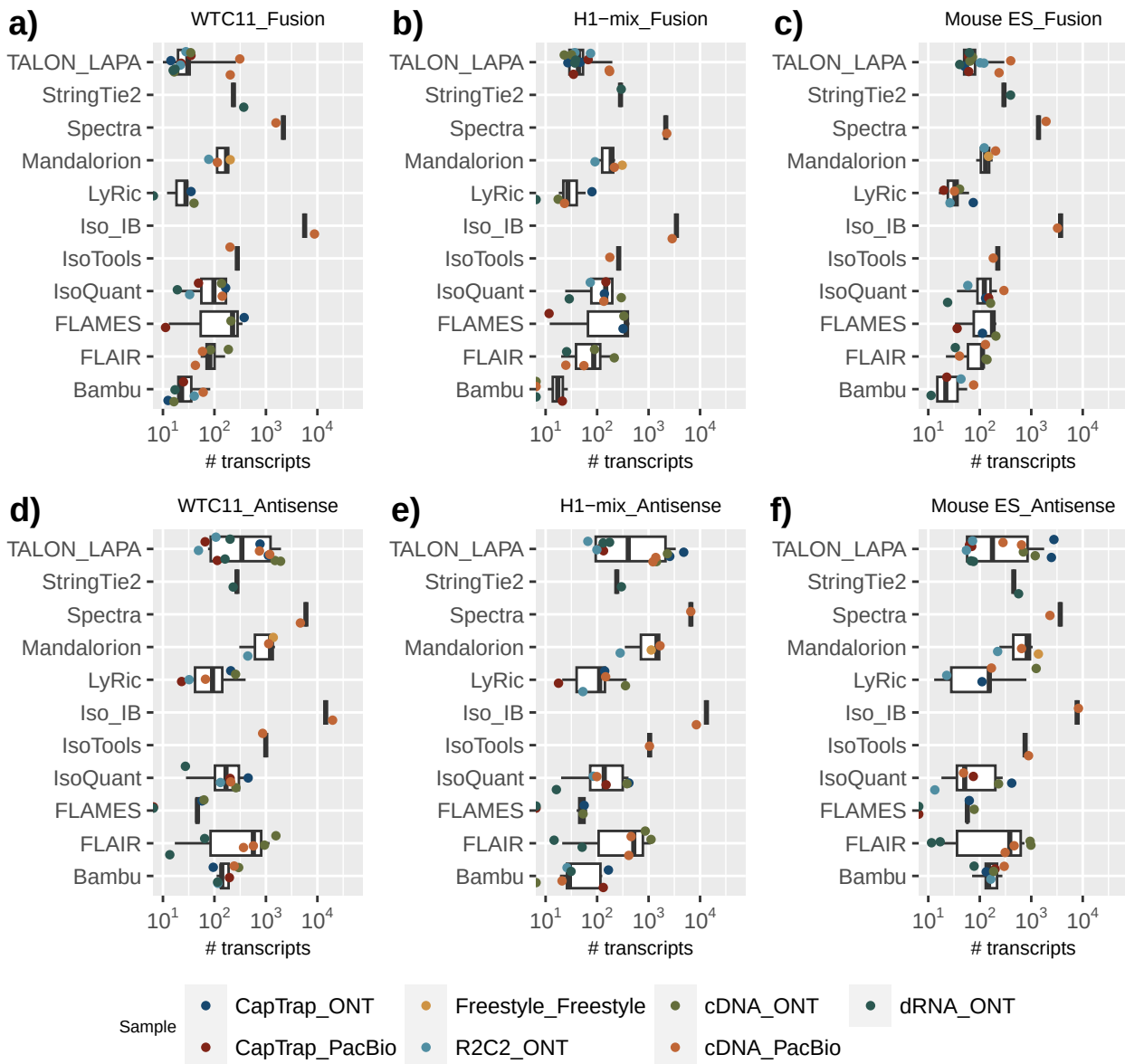
Extended Data Fig. 22. Number of Fusion and Antisense by sequencing platform and library preparation. a-c) Fusion. d-f) Antisense.
