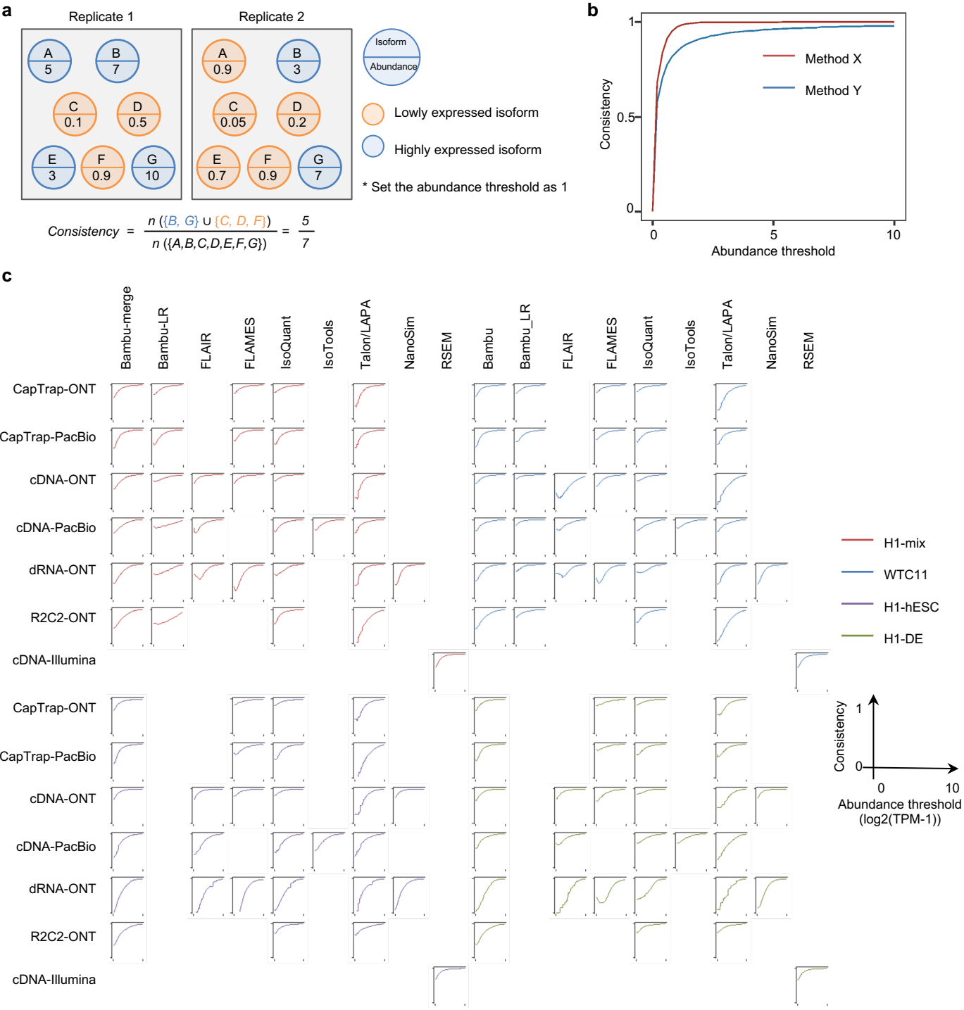
Extended Data Fig. 55. Overall evaluation results of consistency on real data with multiple replicates.
