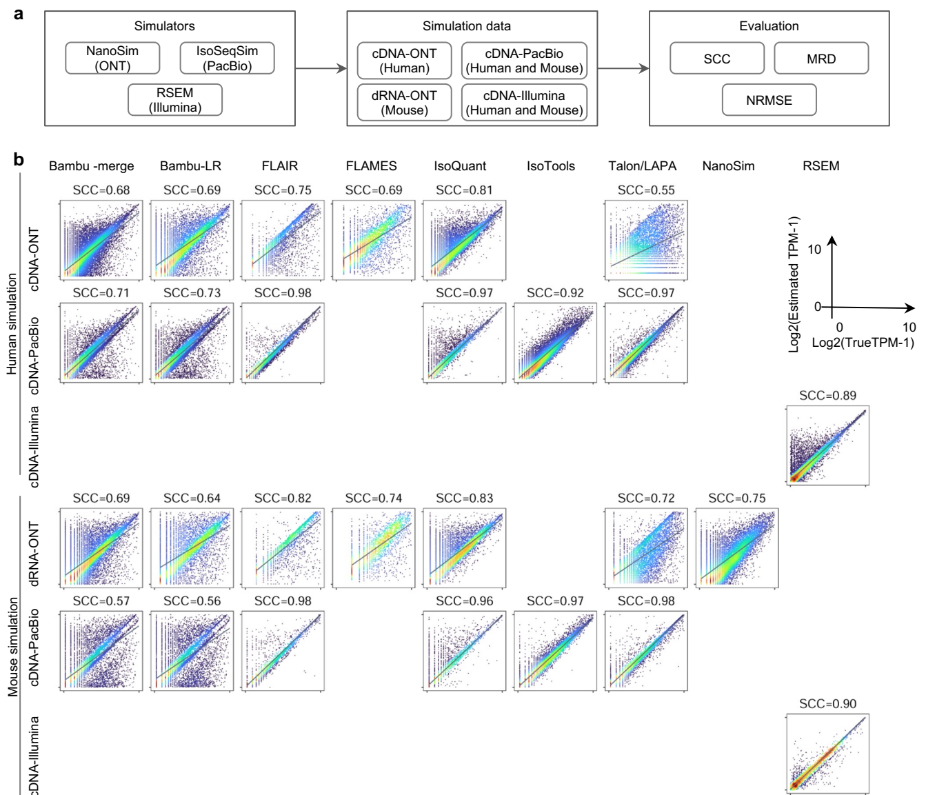
Extended Data Fig. 59. Performance evaluation on simulation data.
