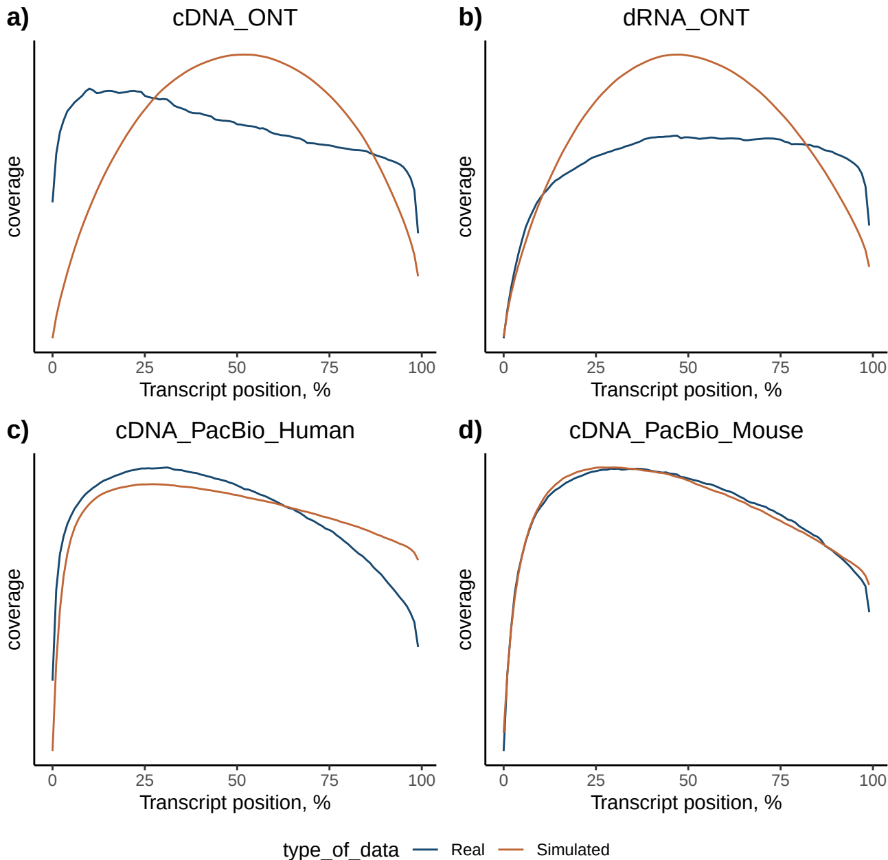
Extended Data Fig. 44. Comparison of long-read transcript coverage between real and simulated datasets.
