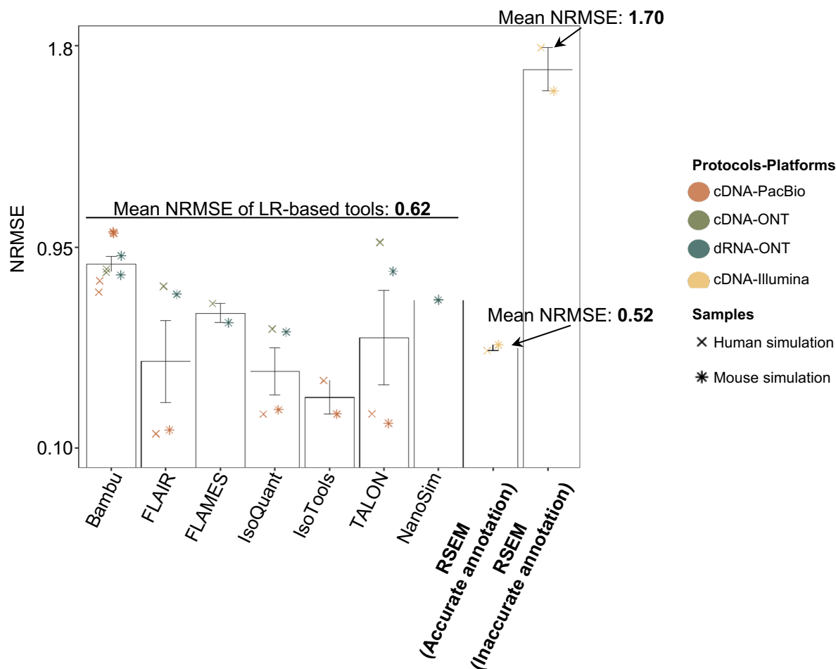
Extended Data Fig. 60. Impact of annotation accuracy on transcript quantification. We assessed the performance of RSEM and LR-based tools (Bambu, FLAIR, FLAMES, IsoQuant, IsoTools, TALON, and NanoSim) with different annotations. The NRMSE metric was used to evaluate their performance on simulated data for human and mouse. For LR-based tools, the transcript quantification annotations were derived from sample-specific annotations identified by the participant using long-read RNA-seq data. As for RSEM, we present quantification results based on two annotations: a completely accurate annotation (i.e., the ground truth transcripts generated by the simulation data) and an inaccurate annotation (i.e., the common GENCODE reference annotation, which contains numerous false negative and false positive transcripts specific to the sample).
