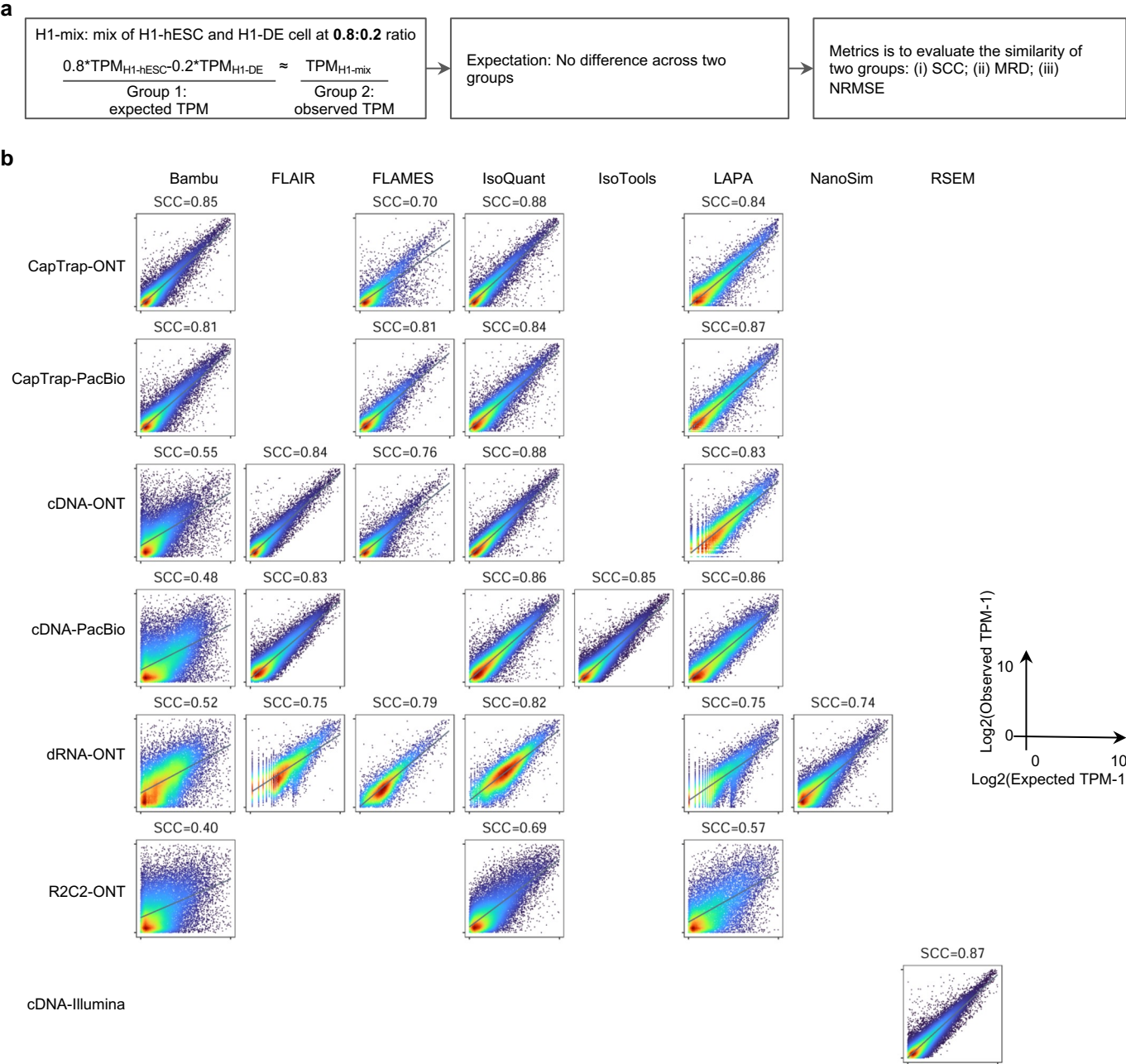
Extended Data Fig. 57. Performance evaluation on cell mixing experiment.
