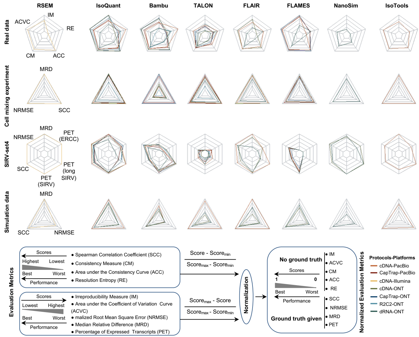
Extended Data Fig. 53. Radar plot of overall evaluation results of 8 quantification tools with 7 protocols-platforms on 4 data scenarios: real data with multiple replicates, cell mixing experiment, SIRV-set4 data and simulation data. To display the evaluation results more effectively, we normalized all metrics to 0-1 range: 0 corresponds to the worst performance and 1 corresponds to the best performance.
