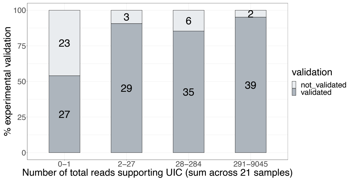
Extended Data Fig. 68. Fraction of validated transcripts as a function of the total numbers of long reads that were observed across the 21 library preparations (e.g., PacBio cDNA, ONT cDNA, PacBio CapTrap).
