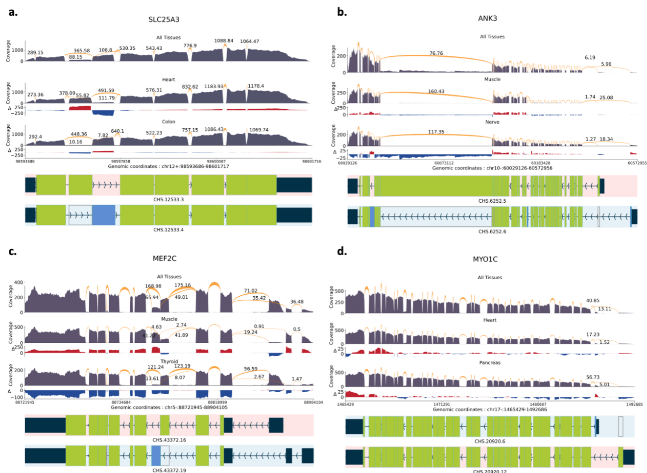
Figure 3: Sashimi plots with normalized coverage and junction values from GTEx samples of CHES 3 project. Only the relevant isoforms and junction values are included for readability. The normalized coverage values for each tissue were subtracted from the normalized coverage of the entire GTEx dataset, and the results were illustrated as the \Delta track. a. SLC25A3 DTU event between heart and colon tissues. b. ANK3 DTU event between muscle and nerve tissues. c. MEF2C DTU event between muscle and thyroid tissues. d. MYO1C DTU event between heart and pancreas tissues.
