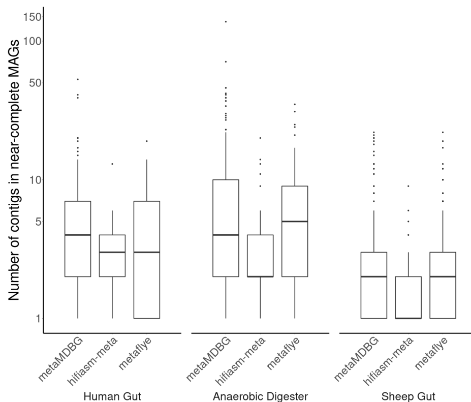
Figure S2: Number of contigs in non-circular near-complete MAGs. The boxplot elements are the median (horizontal bar), 25th and 75th percentiles (box limits Q1 and Q3), Q1-1.5 \times IQR and Q3+1.5 \times IQR (whiskers, IQR=Q3-Q1 ) and outliers. Summary statistics (min, median, mean, max): Human— metaMDBG (1, 4, 6.8, 53); hifiasm-meta (1, 3, 3.1, 13); metaFlye (1, 3, 4.6, 19) : AD— metaMDBG (1, 4, 9.2, 138); hifiasm-meta (1, 2, 3.6, 20); metaFlye (1, 5, 7, 35) : Sheep— metaMDBG (1, 2, 3.3, 22); hifiasm-meta (1, 1, 1.5, 9); metaFlye (1, 2, 2.8, 22). The number of contigs per non-circular MAGs have been extracted from columns ‘AssemblyStatus’ of supplementary File S1.
