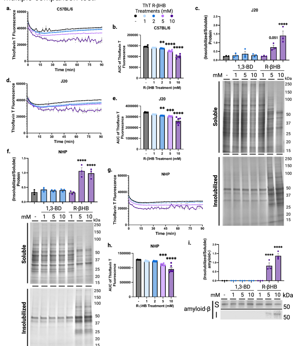
Fig. 3 | β-hydroxybutyrate induces structural remodeling of proteins. a-b, Total protein aggregation kinetics monitored via Thioflavin T fluorescence in mouse soluble cytosolic brain proteins treated with 1-10 mM of R-βHB from 24 month wild-type male, (a) timecourse and (b) area under the curve. c, Imperial stain of 4 month male J20
