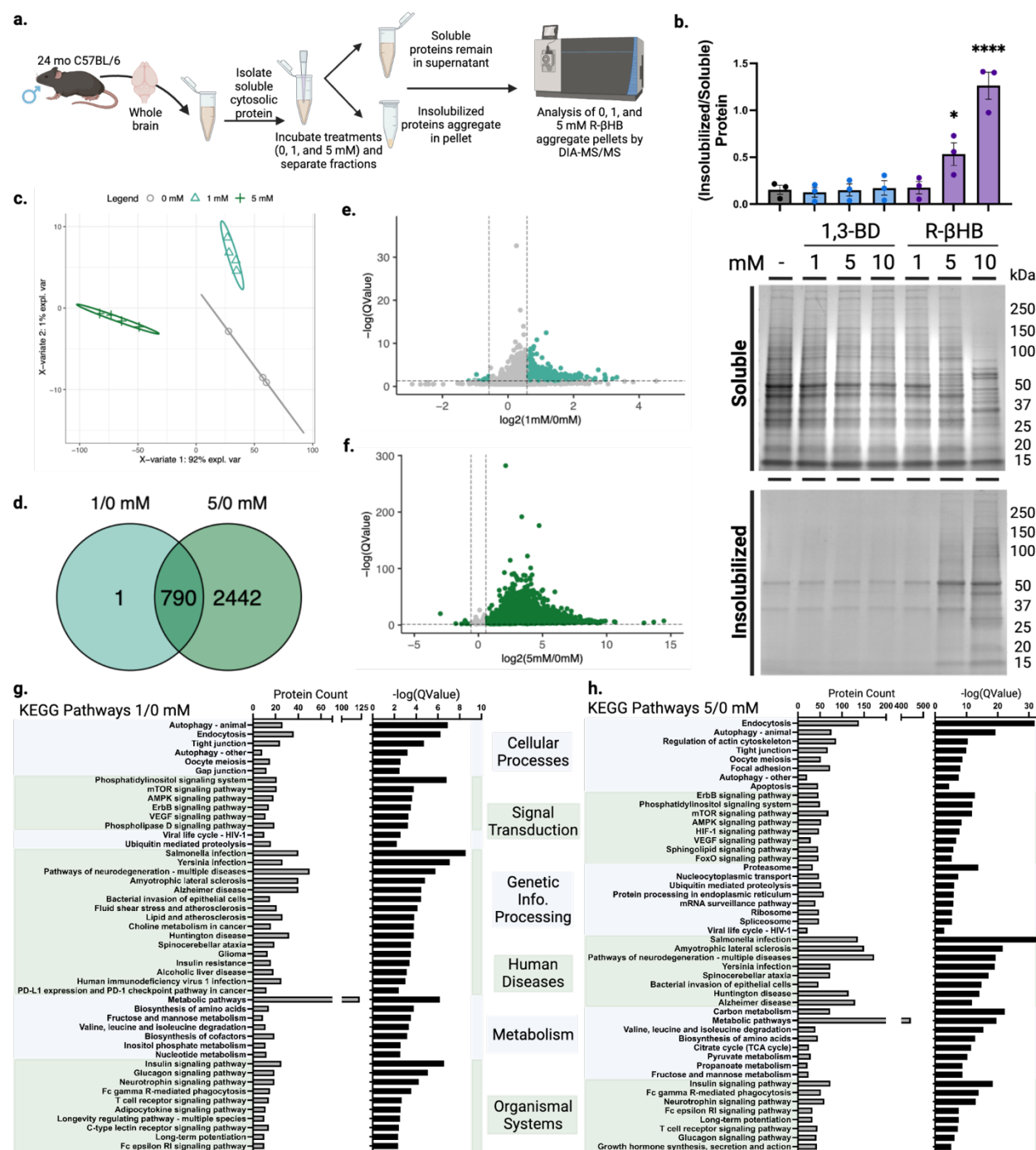
Fig. 2 | \beta -hydroxybutyrate remodels the older C57BL/6 mouse brain proteome ex vivo via insolubilization of targets. a , Schematic of experimental procedures. b , Imperial staining and quantification of 24 month male wild-type mouse soluble cytosolic brain proteins which remain soluble or are insolubilized after treatment with 1-10 mM of R- \beta HB and 1-10 mM of 1,3-BD. c , Partial least squares-discriminant analysis (PLS-DA) of clustering of 0, 1, and 5 mM R- \beta HB proteomic samples. d , Venn diagram comparing target proteins in 1/0 mM and 5/0 mM R- \beta HB proteomics samples. e-f , Volcano plots of (e) 1/0 mM and (f) 5/0 mM R- \beta HB proteomic samples. g-h , Results from clusterProfiler
