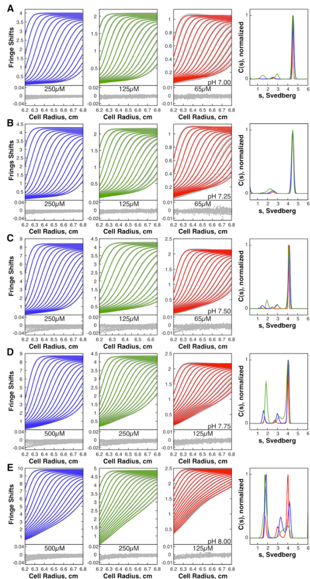
Figure 4. Sedimentation velocity experiments over a range of pH values can be fit with a three-state association model AT_3 \leftrightarrow (AT_3)_2 \leftrightarrow AT_{12} . Interference fringe shifts (gray dots) are globally fit across three AT concentrations (first three columns). Fits provided by the mechanistic model are in blue, green, and red lines. Only every tenth scan is shown. Residuals are below the data. Fourth column, sedimentation coefficient distributions with blue, red and green corresponding to the concentrations on the left, at pH 7.00 (A), pH 7.25 (B), pH 7.50 (C), pH 7.75 (D), and pH 8.00 (E).
