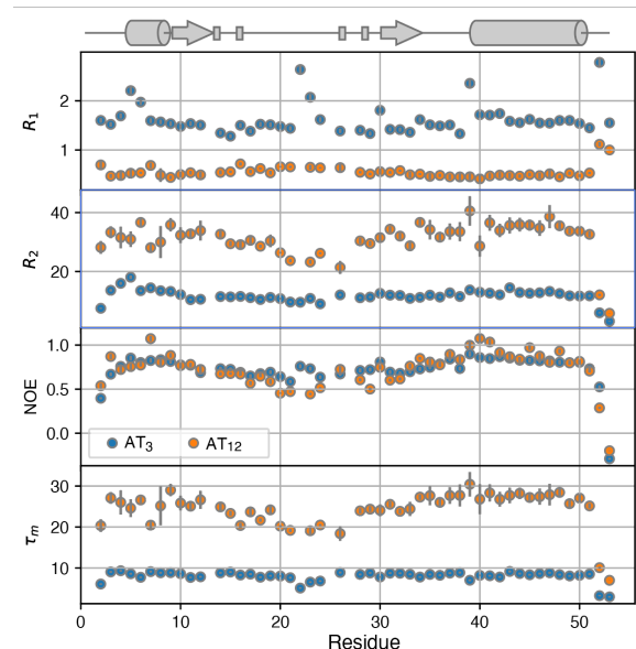
Figure 9. Amide 15 N relaxation rates for trimeric and dodecameric AT reveal differences in overall correlation and local dynamics. Relaxation rates were measured at 600 MHz, 55°C. Local correlation times were computed from the R_2/R_1 ratios {Palmer}. Secondary structures and location of metal ligands are indicated schematically above.
