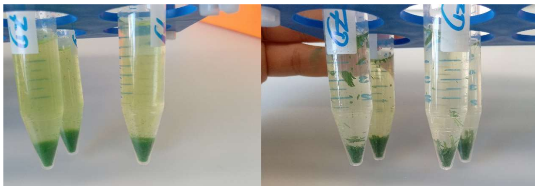
Fig. 3: Comparison of ground flash-frozen (left) versus air-dried (right) leaf tissue following the same pulverization procedures.
