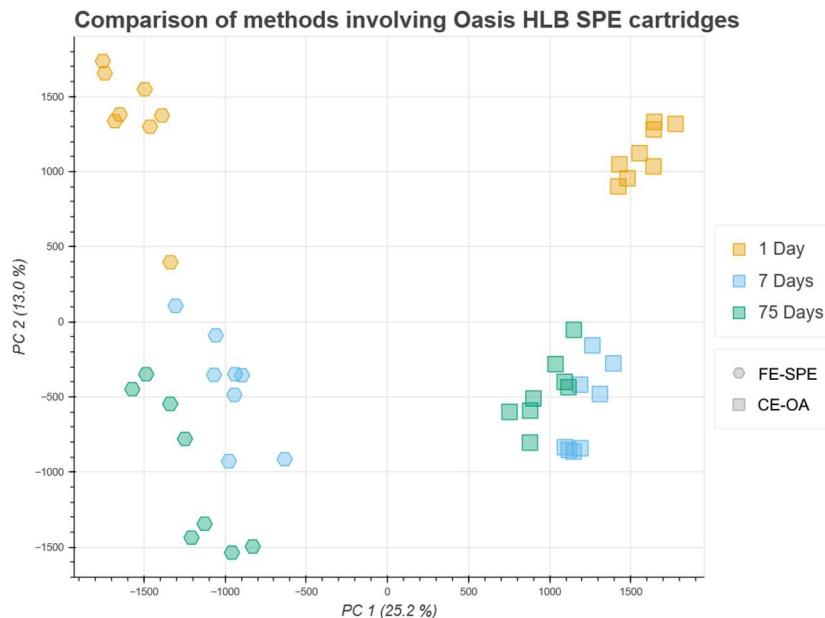
Fig. 7: Principal component analysis of samples stored on an SPE cartridge (CE-OA, squares) and samples prepared by SPE and dried down for storage (FE-SPE, hexagons). Samples stored at 30 °C are not included and FE-SPE samples stored for 28 days were removed as there was no CE-OA counterpart for the direct comparison.
