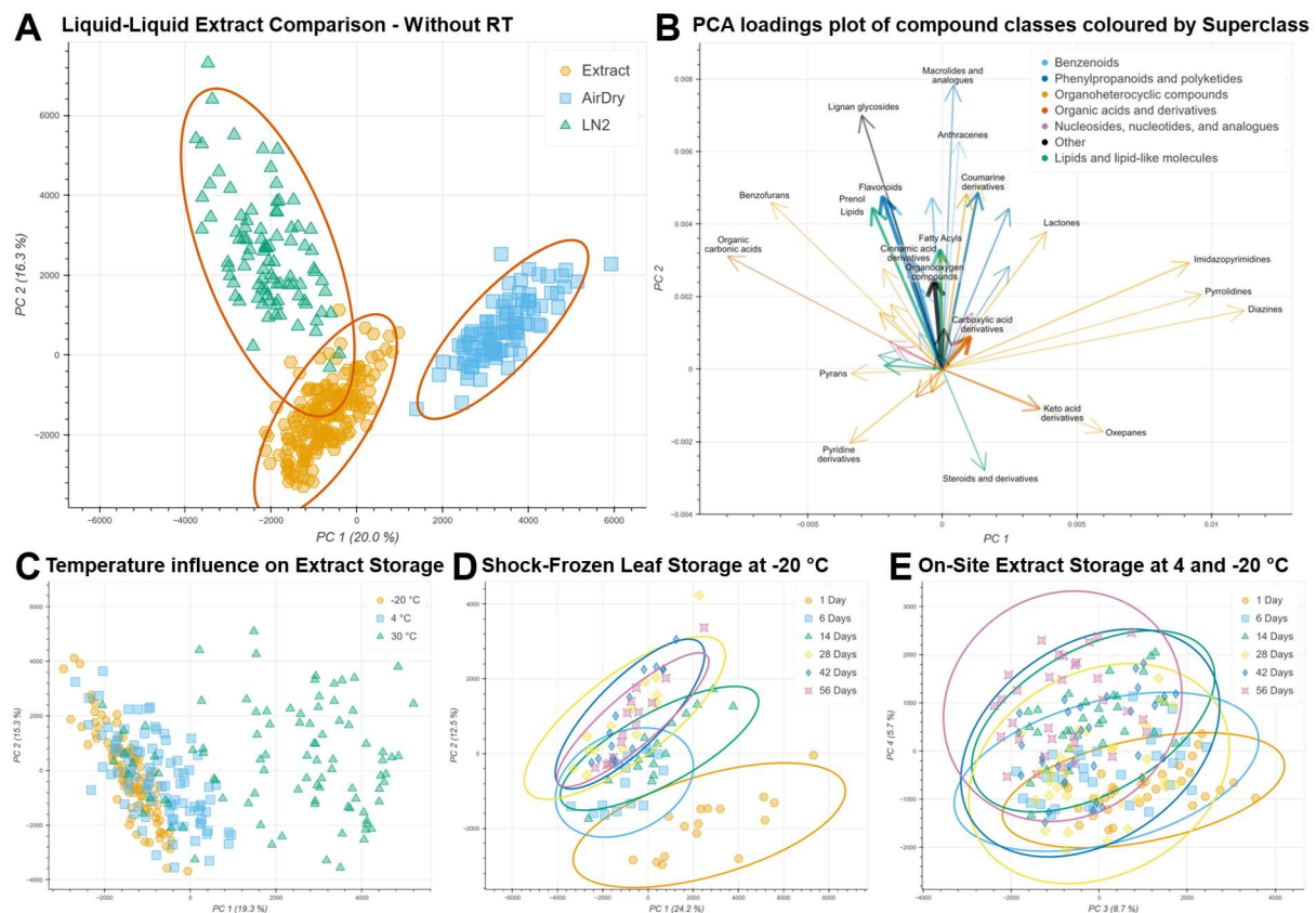
Fig. 5: Principal components analysis (PCA) conducted on metabolite profiles of samples extracted and stored under different conditions: (A) LLE of differently handled leaf tissue samples, (B) compound class impact on the separation of 5A, arrow width indicates number of compounds of each class in a range between 5 and 199 compounds, (C) influence of storage temperature on the metabolite profile shift of LLE extracts (includes all storage timepoints), (D) profile shift over time for frozen storage of shock-frozen leaf tissue, (E) shift of on-site LLE of both -20 °C and 4 °C.
