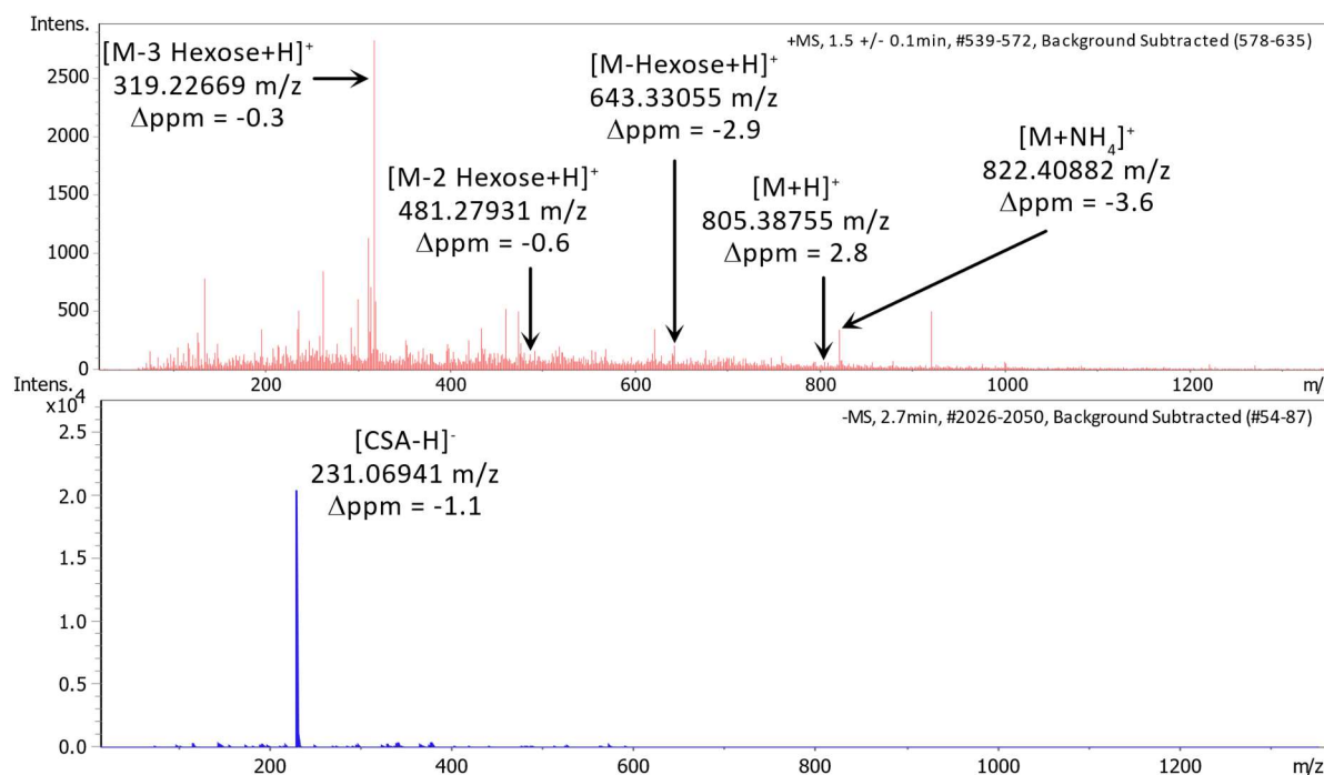
Fig. 2: Comparison of the full scan MS spectrum of the internal standards stevioside (red, A) and camphorsulphonic acid (CSA, blue, B) with signal annotation of matching m/z ratios.
