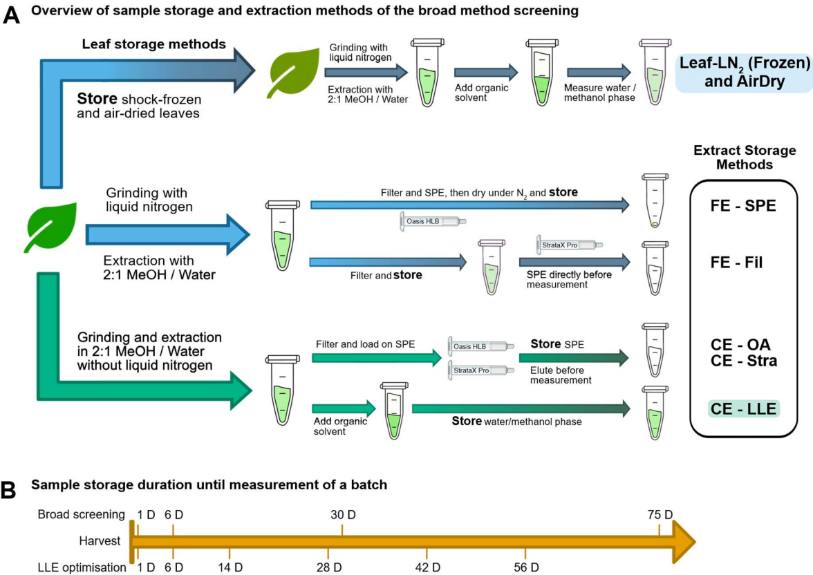
Fig. 1: Overview of the evaluated sample extraction and storage methods (A). Blue arrows indicate extractions where liquid nitrogen was used during homogenisation (FE = Frozen Extraction), while green arrows indicate that no liquid nitrogen was used (CE = Crude Extraction). Bright colours indicate pre-storage processing, dark colours show sample preparation done after the storage period. Only the top pathway includes methods where leaf tissue is stored, either frozen or air-dried, the other pathways show the various leaf extract storage methods, which were prepared within 30 hours of harvest. The highlighted methods were later used during the LLE optimisation, where CE-LLE is referred to as “On-Site Extract storage”. The timeline (B) shows the evaluation time points of the broad method screening and the LLE Optimisation.
