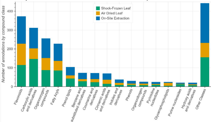
Compound classes annotated for the Methods of the LLE Optimisation
