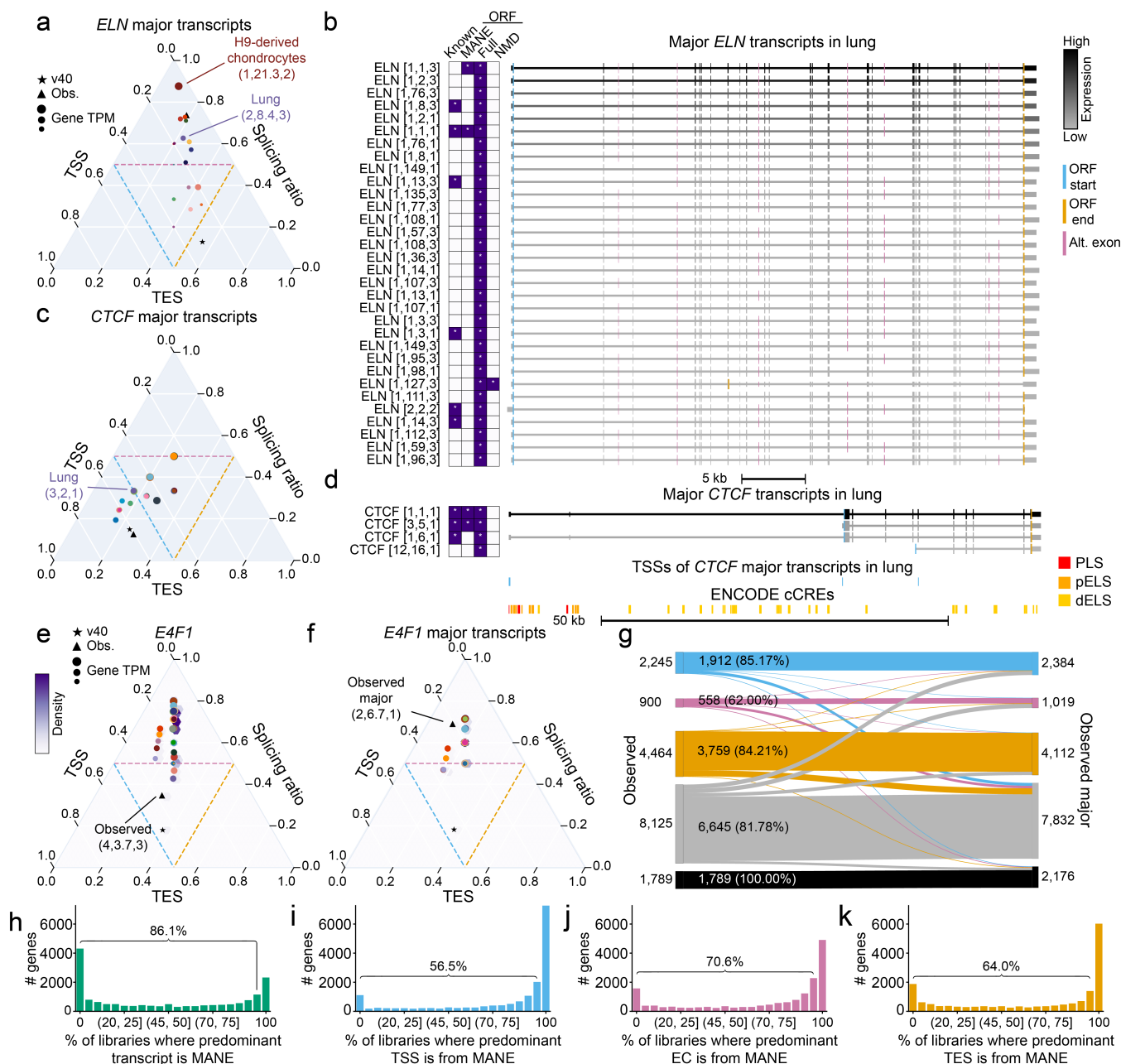
Figure 4. Sample-specific and global changes in predominant and major transcript isoform usage. a , Gene structure simplex for major transcripts of ELN . Gene triplets with splicing ratio for lung and H9-derived chondrocytes labeled. Simplex coordinates for the GENCODE v40 and observed major set are labeled. b , Major transcripts of ELN expressed \geq 1 TPM in lung colored by expression level in TPM. Alternative exons that differ between transcripts are colored pink. c , Gene structure simplex for major transcripts of CTCF . Gene triplets with splicing ratio for lung labeled. Simplex coordinates for the GENCODE v40 and observed major set are labeled. d , From top to bottom: Major transcripts of CTCF expressed \geq 1 TPM in lung, TSSs of CTCF major transcripts expressed \geq 1 TPM in lung, ENCODE cCREs colored by type. e , Gene structure simplex for E4F1 . Gene triplet with splicing ratio for observed E4F1 transcripts labeled. Simplex coordinates for the GENCODE v40 and observed set also shown for E4F1 . f , Gene structure simplex for major transcripts of E4F1 . Gene triplet with splicing ratio for observed major E4F1 transcripts labeled. Simplex coordinates for the GENCODE v40 and observed major set also shown for E4F1 . g , Sector assignment change and conservation for protein coding genes in the human ENCODE LR-RNA-seq dataset between the observed set of gene triplets (left) and the observed major set of gene triplets (right). Percent of genes with the same sector between both sets labeled in the middle. h-k , Percentage of libraries where a gene with an annotated MANE transcript is expressed and the MANE h , transcript i , TSS j , EC k , TES is the predominant transcript or triplet feature.
