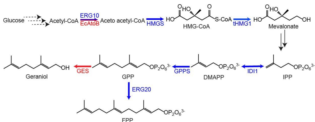
Figure 1. Yarrowia lipolytica geraniol biosynthesis pathway. The blue arrows indicate native enzymes and red arrows indicate heterologous enzymes. ERG10/AtoB is acetyl-CoA acetyltransferase, HMGS is HMG synthase, HMG is β-Hydroxy β-methylglutarate, tHMGI is truncated HMG-CoA reductase, IPP is isopentenyl 5-pyrophosphate, IDI1 is IPP isomerase, DMAPP is dimethylallyl 5-pyrophosphate, GPPS is geranyl pyrophosphate synthase, GES is geraniol synthase.
