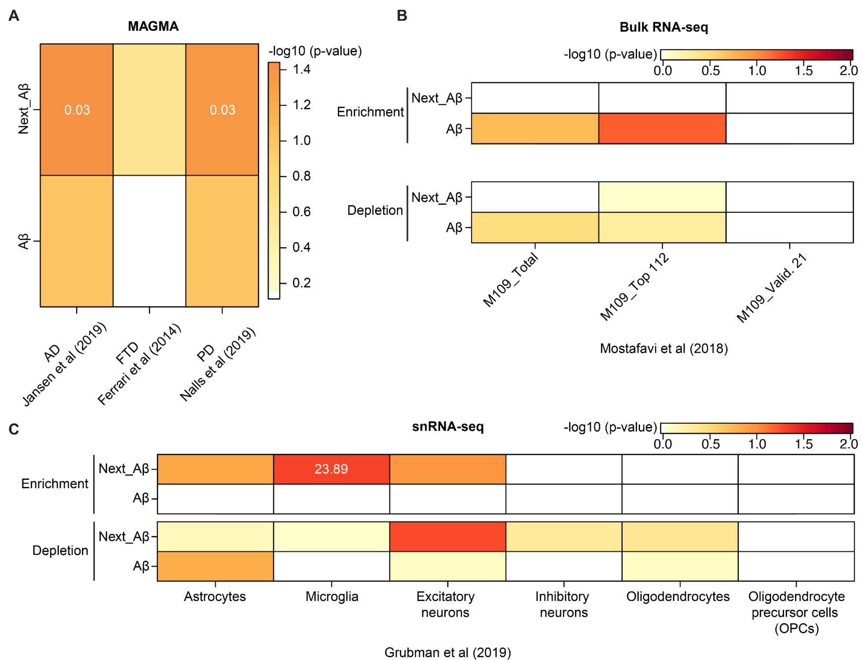
Figure S13. Enrichment of neurodegeneration- and dementia-related gene sets in A \beta -associated microenvironments.
