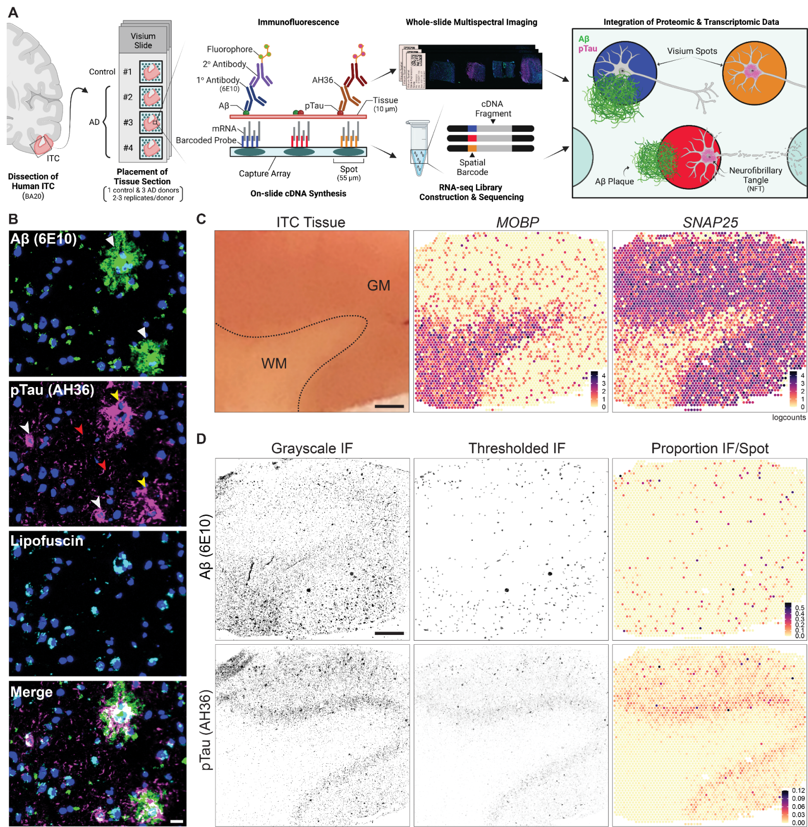
Fig.1 Spatial transcriptomics combined with immunodetection of Aβ and pTau in the human inferior temporal cortex (ITC).
