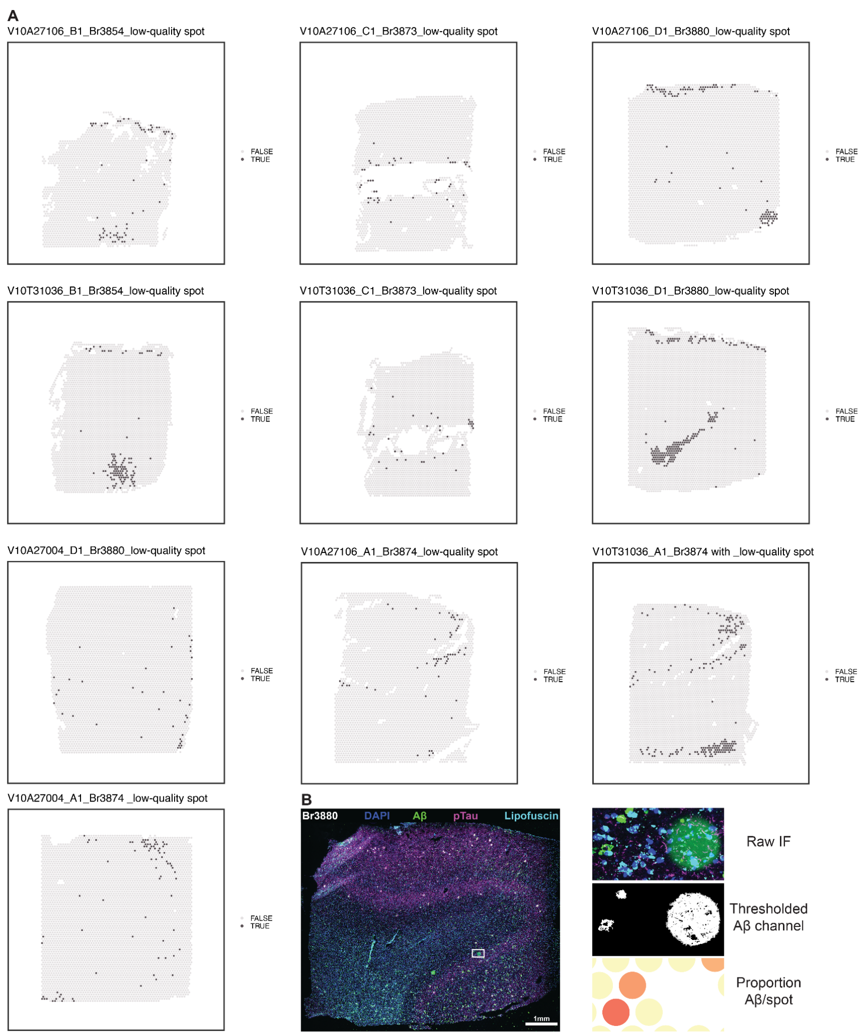
Figure S9. Spot-level quality control of Visium SRT data.
