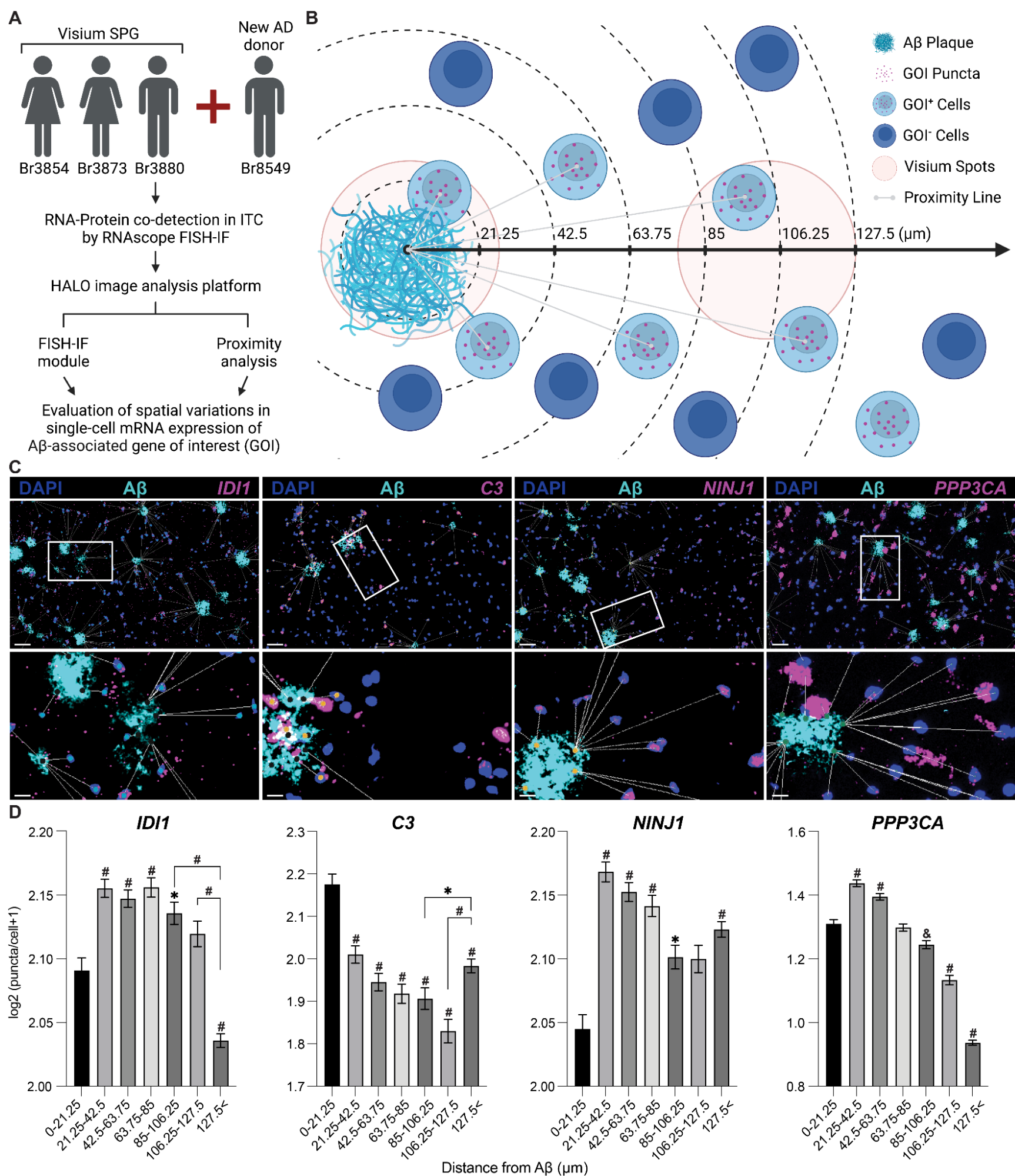
Fig.3 Characterization of A \beta -associated transcriptional signatures at cellular resolution.
