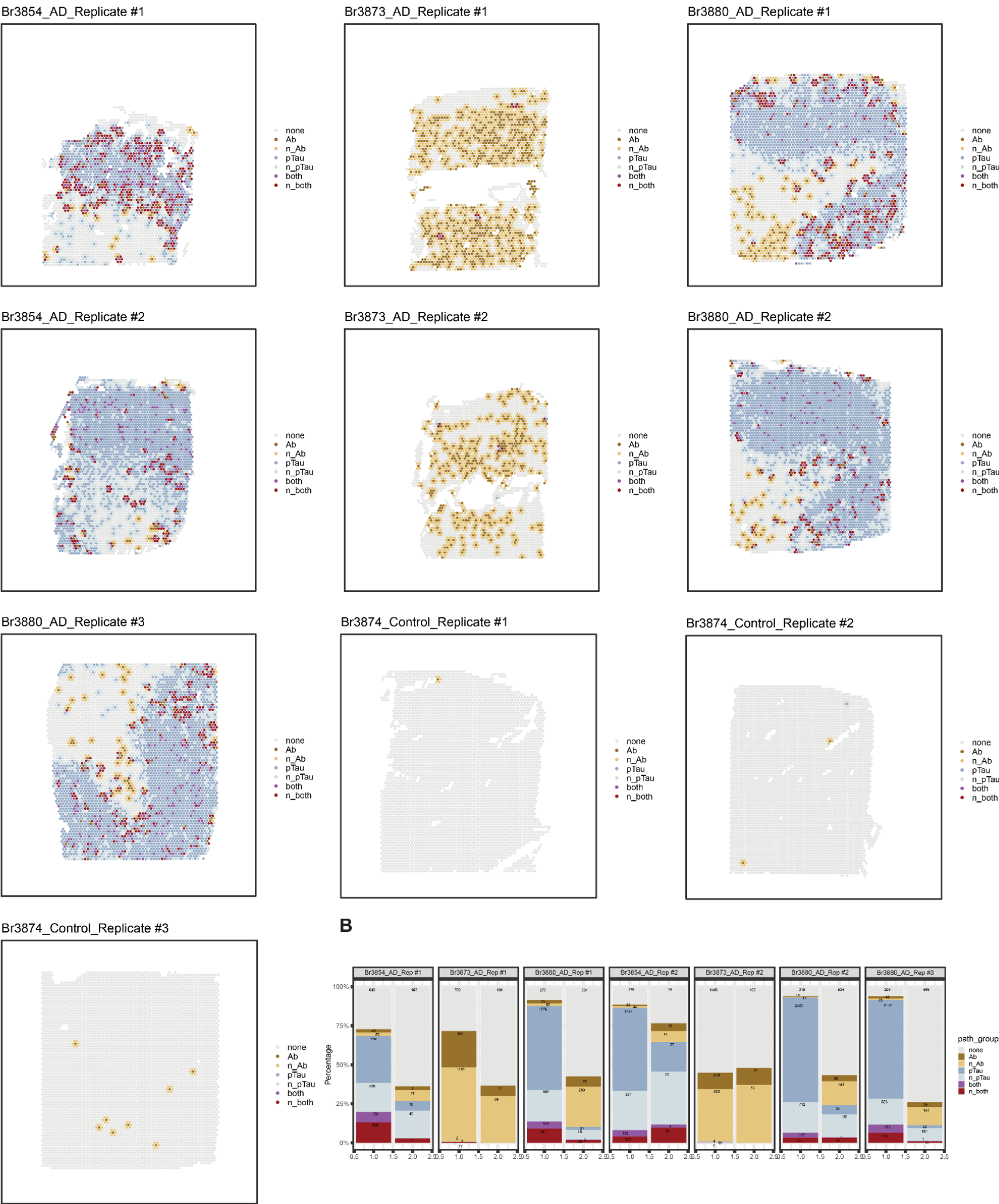
Figure S8. Classification of spots into different AD-related neuropathological categories.
