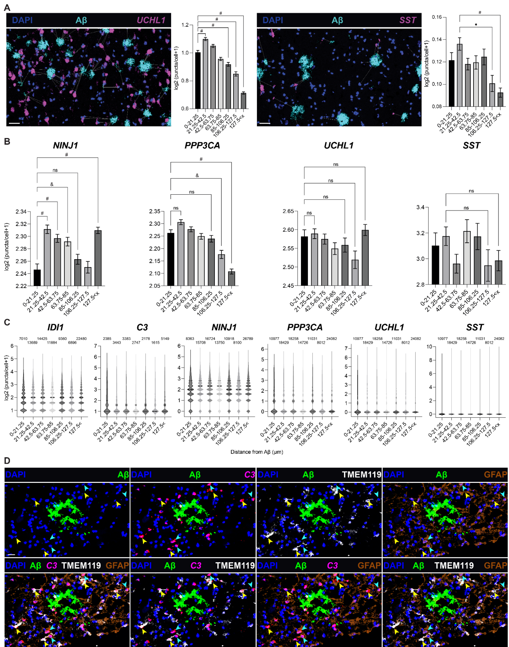
Figure S16. Validation of quantification strategies of Aβ-associated transcriptional signatures at cellular resolution.
