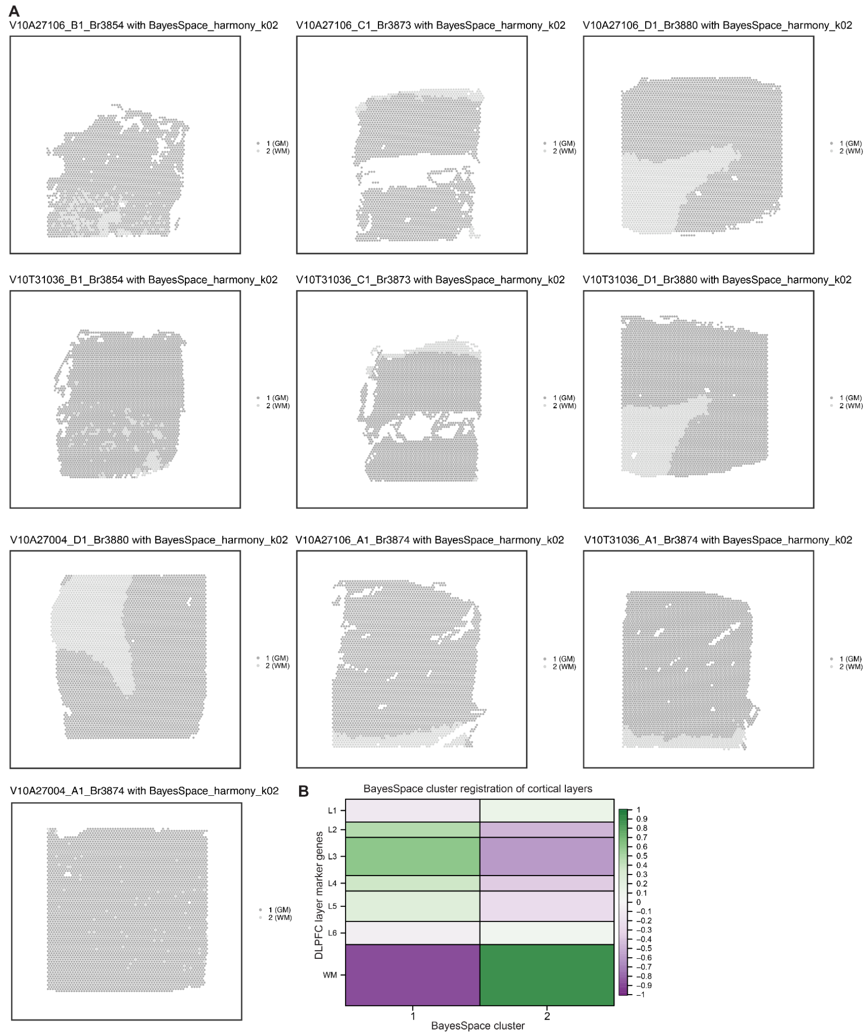
Figure S11. Unsupervised clustering with BayesSpace separates white and gray matter clusters in all tissue sections.
