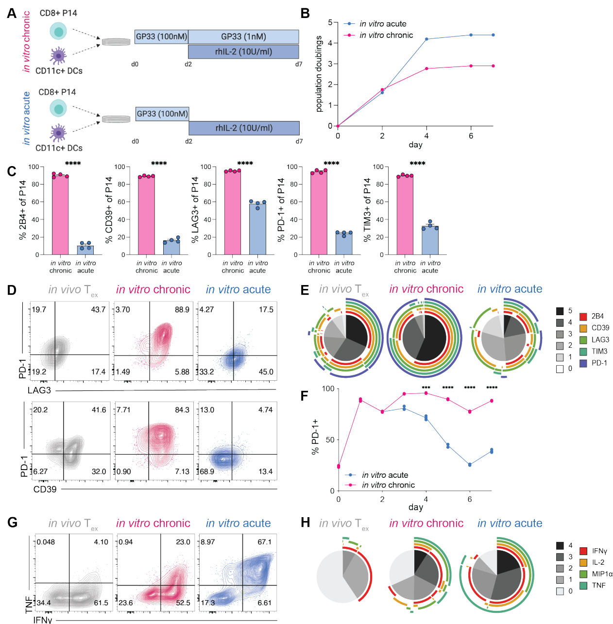
Fig. 1. Chronic antigenic stimulation in vitro induces key features of T_{ex} (A) Experiment schematic of chronic and acute stimulation of P14 cells in vitro . (B) Cell expansion during chronic and acute stimulation in vitro . (C) Percent expression of IRs by chronically and acutely stimulated P14 cells (gated on CD44^{hi} CD8^{+} live singlets); two technical replicates of two biological replicates shown. Significance calculated by unpaired two-tailed t test; **** p < 0.0001 . (D) Representative flow cytometry data and (E) SPICE analysis of IR co-expression by in vivo T_{ex} (LCMV-CI13 30dpi), in vitro chronically stimulated P14 cells, and in vitro acutely stimulated P14 cells (gated on CD44^{hi} CD8^{+} live singlets). (F) Longitudinal PD-1 expression on in vitro chronically and acutely stimulated P14 cells. Representative of 2 experiments; significance calculated by paired two-tailed t test; * p < 0.05 , ** p < 0.01 , *** p < 0.001 , **** p < 0.0001 . (G) Representative flow cytometry data and (H) SPICE analysis of co-production of effector cytokines in in vivo T_{ex} (LCMV-
